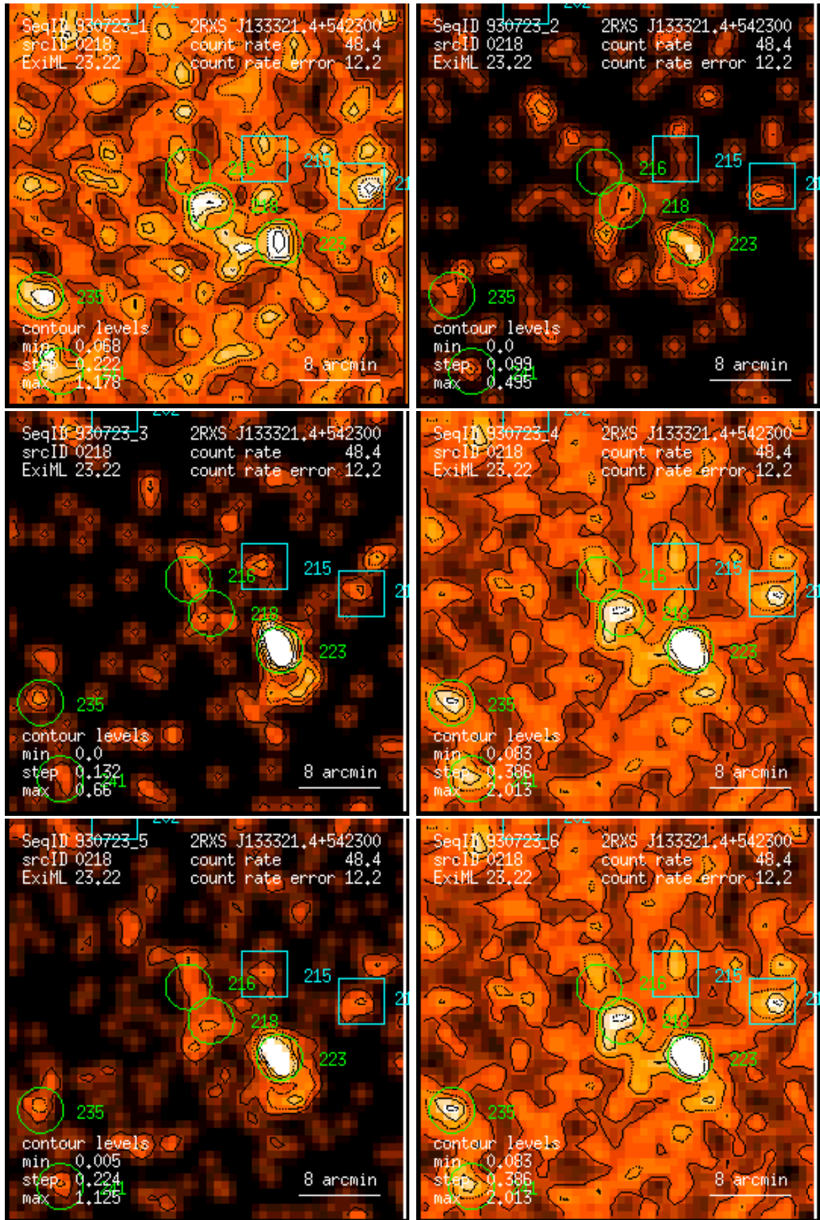
Figure 218: RASS 930723: detection 0218: band rate images, Gaussian filter: (1) PSPC channels 11 – 41, (2) 52 – 90, (3) 91 – 201, (4) 11 – 235, (5) 52 – 201, (6) 11 – 201. Broad band rates in counts/ks. Band rate contour levels in counts/ks/arcmin 2 .
