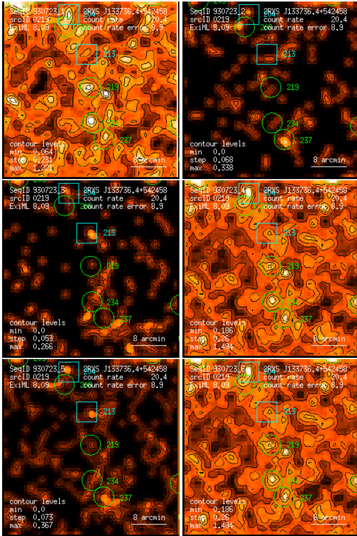
Figure 219: RASS 930723: detection 0219: band rate images, Gaussian filter: (1) PSPC channels 11 – 41, (2) 52 – 90, (3) 91 – 201, (4) 11 – 235, (5) 52 – 201, (6) 11 – 201. Broad band rates in counts/ks. Band rate contour levels in counts/ks/arcmin 2 .
