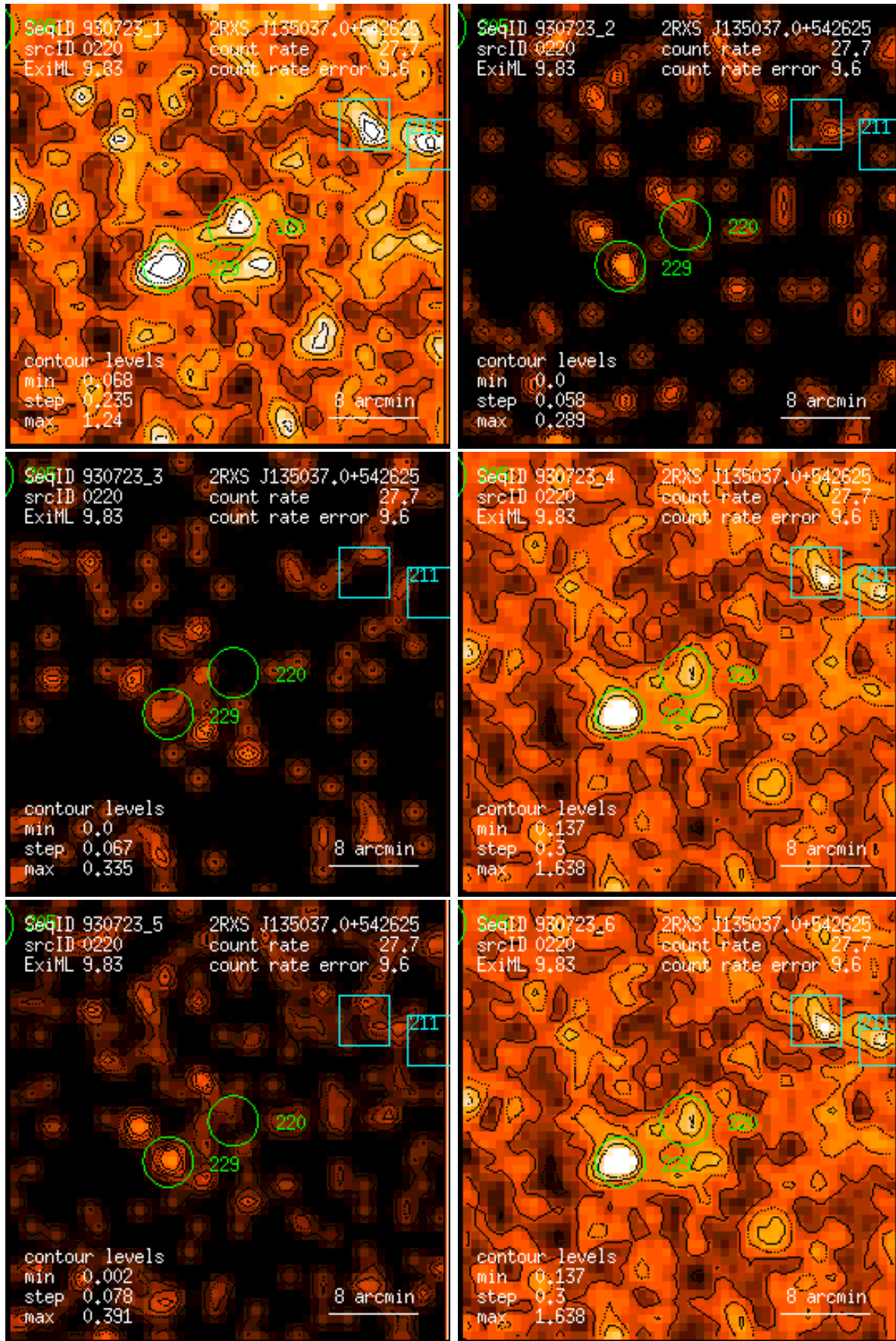
Figure 220: RASS 930723: detection 0220: band rate images, Gaussian filter: (1) PSPC channels 11 – 41, (2) 52 – 90, (3) 91 – 201, (4) 11 – 235, (5) 52 – 201, (6) 11 – 201. Broad band rates in counts/ks. Band rate contour levels in counts/ks/arcmin 2 .
