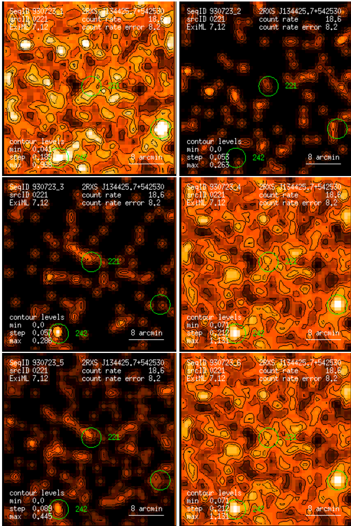
Figure 221: RASS 930723: detection 0221: band rate images, Gaussian filter: (1) PSPC channels 11 – 41, (2) 52 – 90, (3) 91 – 201, (4) 11 – 235, (5) 52 – 201, (6) 11 – 201. Broad band rates in counts/ks. Band rate contour levels in counts/ks/arcmin 2 .
