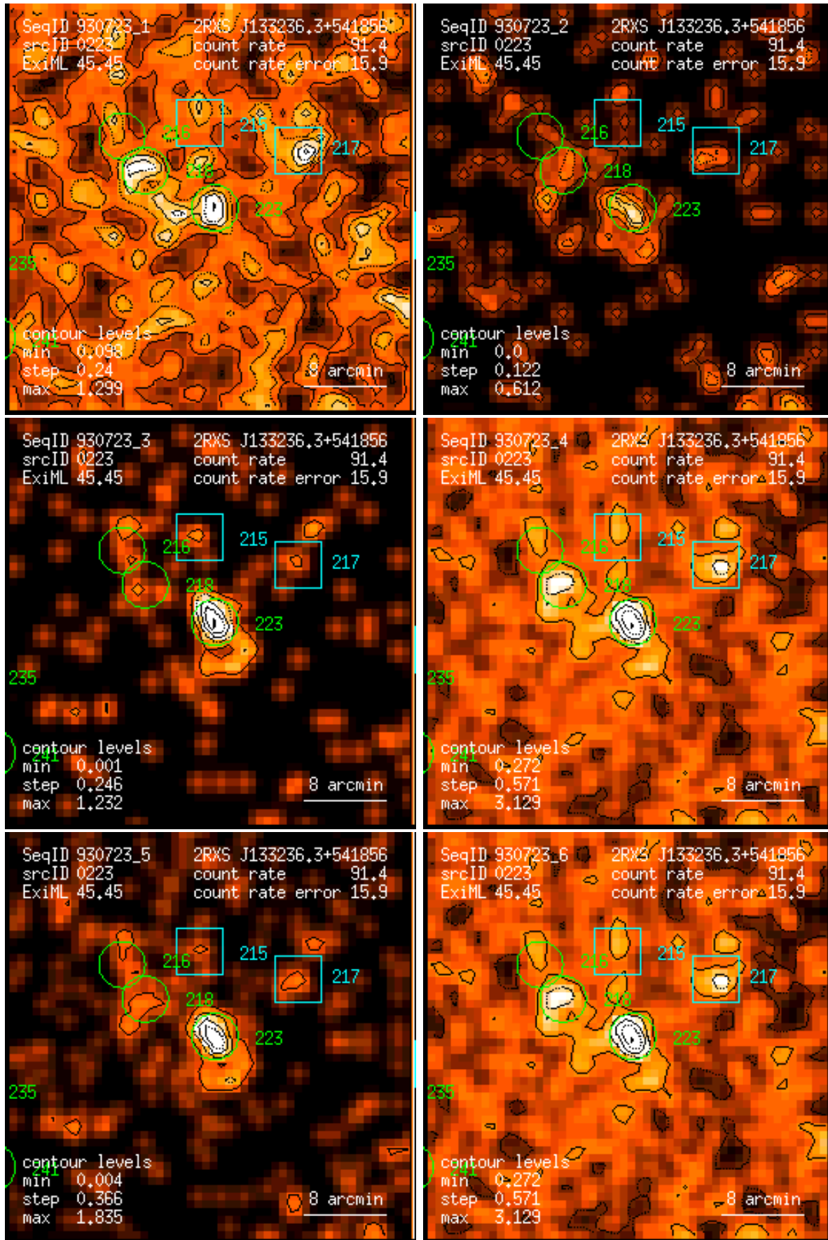
Figure 223: RASS 930723: detection 0223: band rate images, Gaussian filter: (1) PSPC channels 11 – 41, (2) 52 – 90, (3) 91 – 201, (4) 11 – 235, (5) 52 – 201, (6) 11 – 201. Broad band rates in counts/ks. Band rate contour levels in counts/ks/arcmin 2 .
