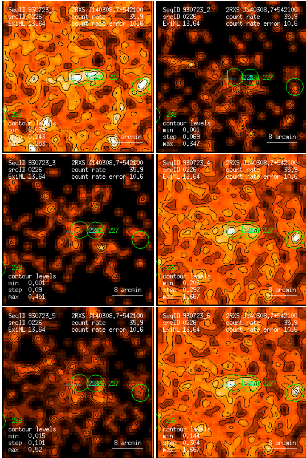
Figure 226: RASS 930723: detection 0226: band rate images, Gaussian filter: (1) PSPC channels 11 – 41, (2) 52 – 90, (3) 91 – 201, (4) 11 – 235, (5) 52 – 201, (6) 11 – 201. Broad band rates in counts/ks. Band rate contour levels in counts/ks/arcmin 2 .
