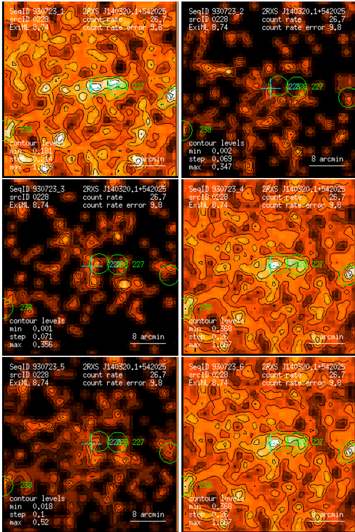
Figure 228: RASS 930723: detection 0228: band rate images, Gaussian filter: (1) PSPC channels 11 – 41, (2) 52 – 90, (3) 91 – 201, (4) 11 – 235, (5) 52 – 201, (6) 11 – 201. Broad band rates in counts/ks. Band rate contour levels in counts/ks/arcmin 2 .
