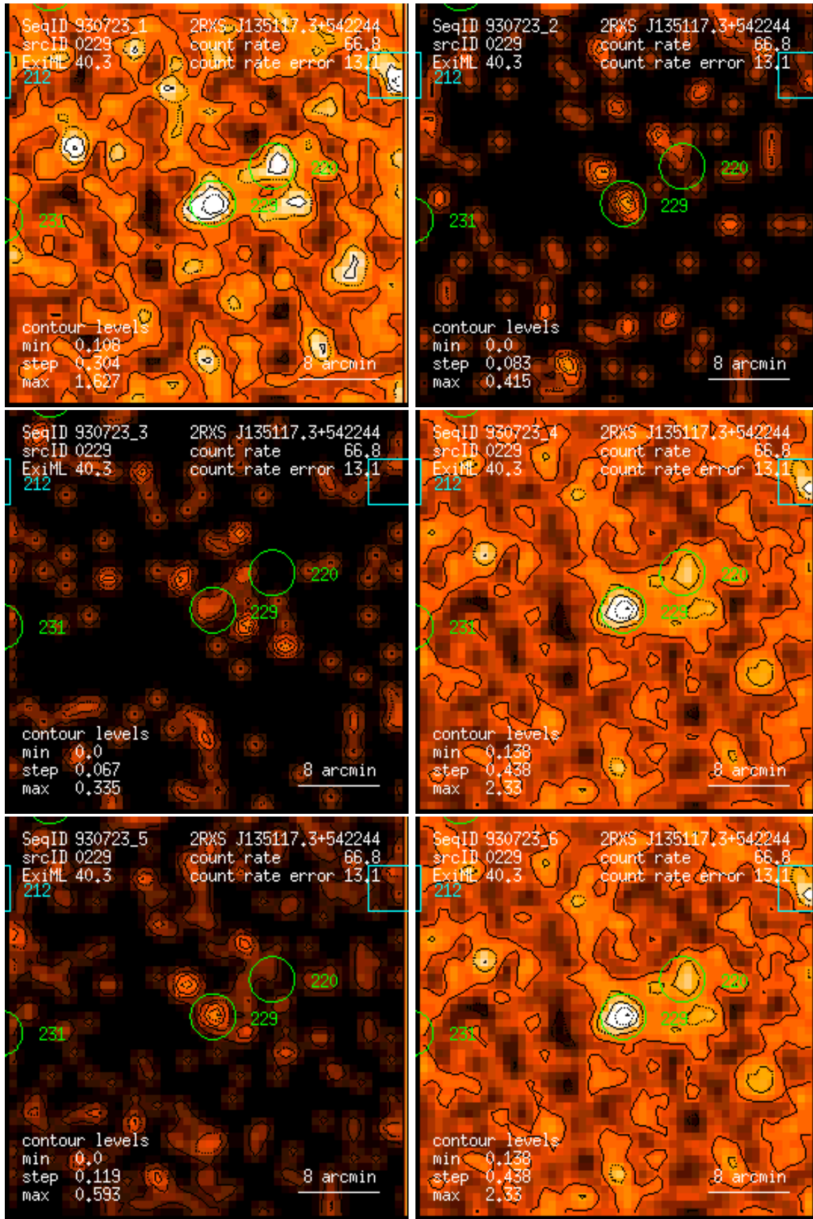
Figure 229: RASS 930723: detection 0229: band rate images, Gaussian filter: (1) PSPC channels 11 – 41, (2) 52 – 90, (3) 91 – 201, (4) 11 – 235, (5) 52 – 201, (6) 11 – 201. Broad band rates in counts/ks. Band rate contour levels in counts/ks/arcmin 2 .
