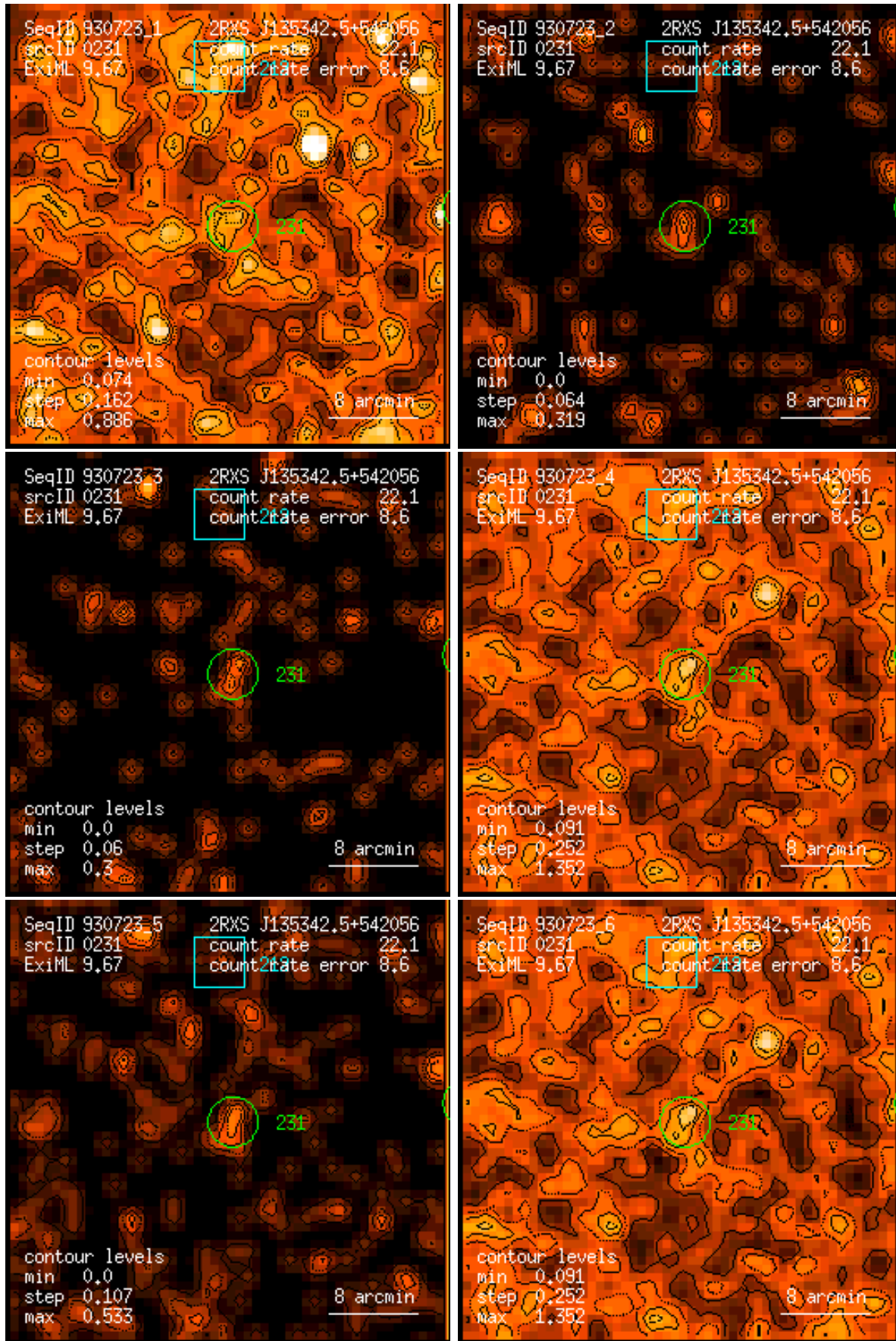
Figure 231: RASS 930723: detection 0231: band rate images, Gaussian filter: (1) PSPC channels 11 – 41, (2) 52 – 90, (3) 91 – 201, (4) 11 – 235, (5) 52 – 201, (6) 11 – 201. Broad band rates in counts/ks. Band rate contour levels in counts/ks/arcmin 2 .
