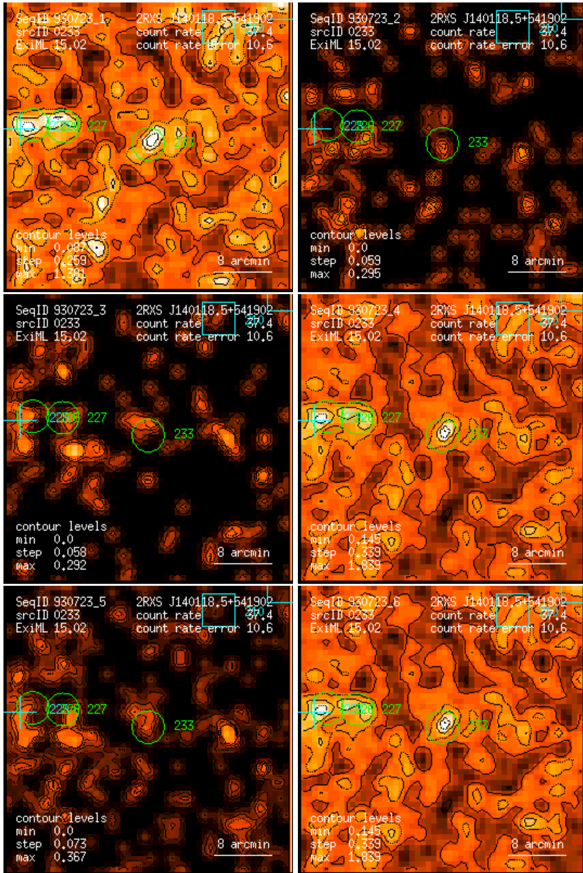
Figure 233: RASS 930723: detection 0233: band rate images, Gaussian filter: (1) PSPC channels 11 – 41, (2) 52 – 90, (3) 91 – 201, (4) 11 – 235, (5) 52 – 201, (6) 11 – 201. Broad band rates in counts/ks. Band rate contour levels in counts/ks/arcmin 2 .
