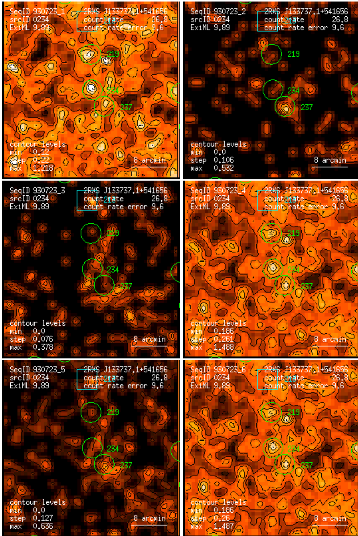
Figure 234: RASS 930723: detection 0234: band rate images, Gaussian filter: (1) PSPC channels 11 – 41, (2) 52 – 90, (3) 91 – 201, (4) 11 – 235, (5) 52 – 201, (6) 11 – 201. Broad band rates in counts/ks. Band rate contour levels in counts/ks/arcmin 2 .
