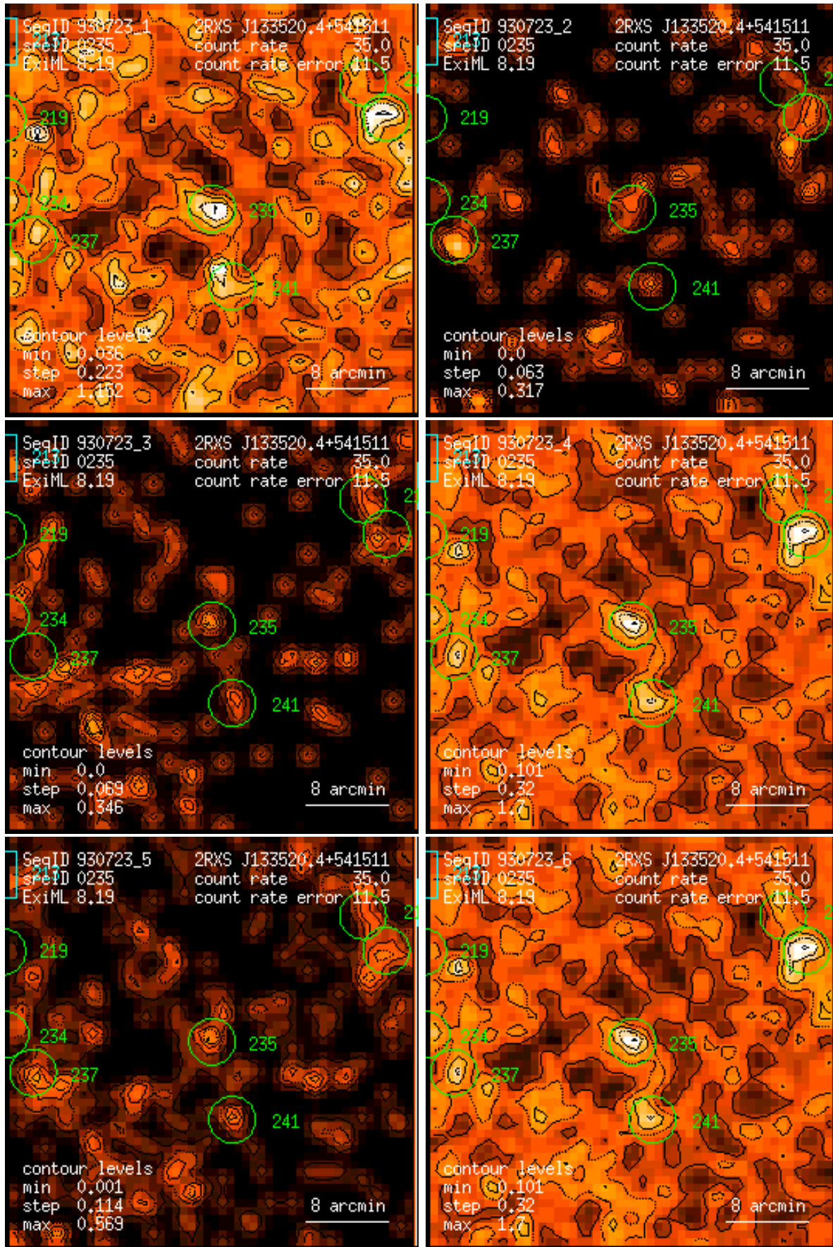
Figure 235: RASS 930723: detection 0235: band rate images, Gaussian filter: (1) PSPC channels 11 – 41, (2) 52 – 90, (3) 91 – 201, (4) 11 – 235, (5) 52 – 201, (6) 11 – 201. Broad band rates in counts/ks. Band rate contour levels in counts/ks/arcmin 2 .
