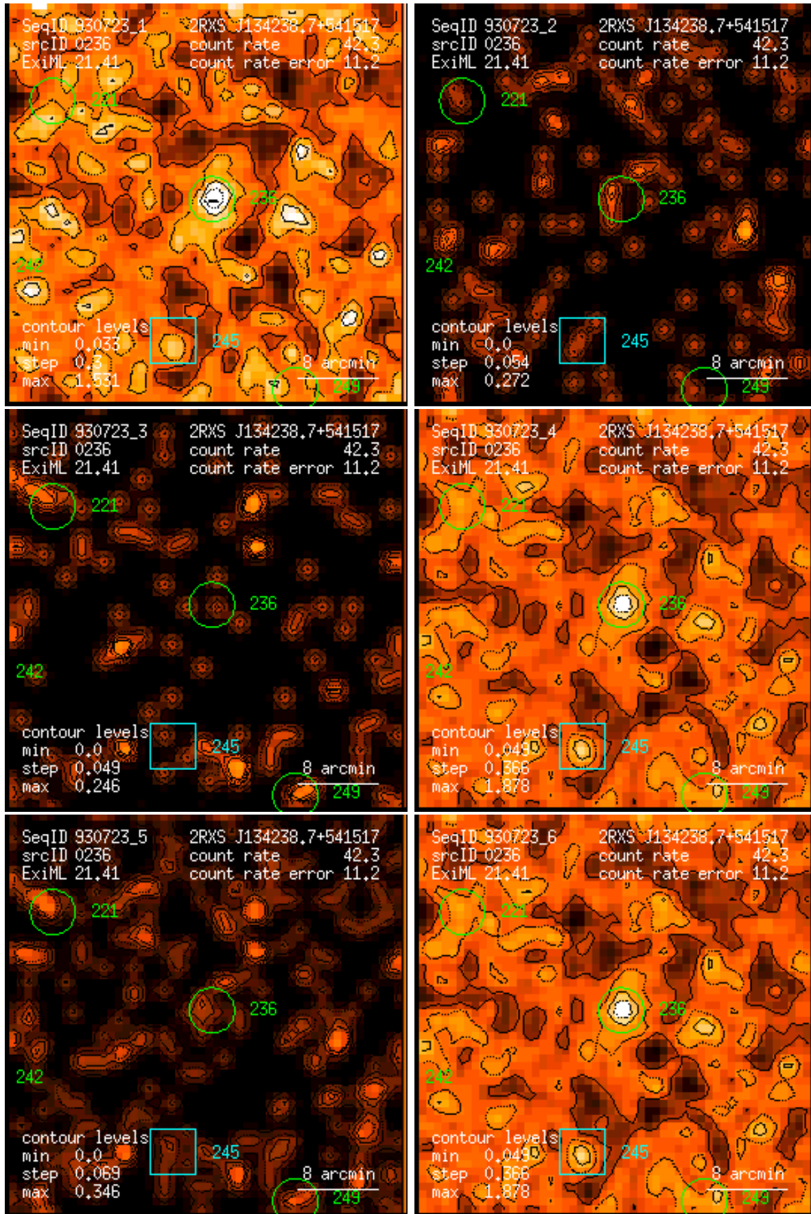
Figure 236: RASS 930723: detection 0236: band rate images, Gaussian filter: (1) PSPC channels 11 – 41, (2) 52 – 90, (3) 91 – 201, (4) 11 – 235, (5) 52 – 201, (6) 11 – 201. Broad band rates in counts/ks. Band rate contour levels in counts/ks/arcmin 2 .
