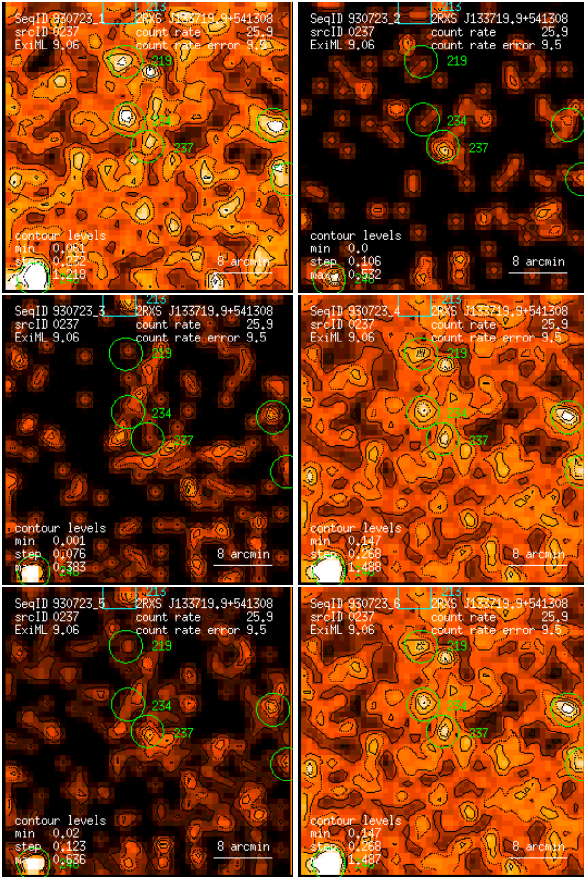
Figure 237: RASS 930723: detection 0237: band rate images, Gaussian filter: (1) PSPC channels 11 – 41, (2) 52 – 90, (3) 91 – 201, (4) 11 – 235, (5) 52 – 201, (6) 11 – 201. Broad band rates in counts/ks. Band rate contour levels in counts/ks/arcmin 2 .
