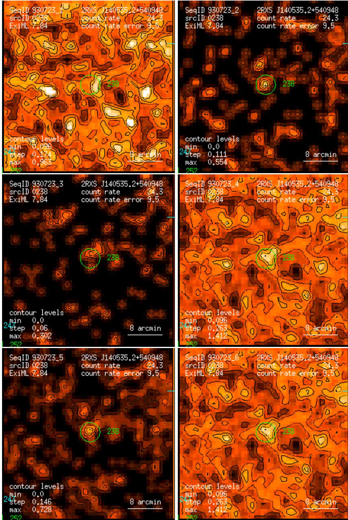
Figure 238: RASS 930723: detection 0238: band rate images, Gaussian filter: (1) PSPC channels 11 – 41, (2) 52 – 90, (3) 91 – 201, (4) 11 – 235, (5) 52 – 201, (6) 11 – 201. Broad band rates in counts/ks. Band rate contour levels in counts/ks/arcmin 2 .
