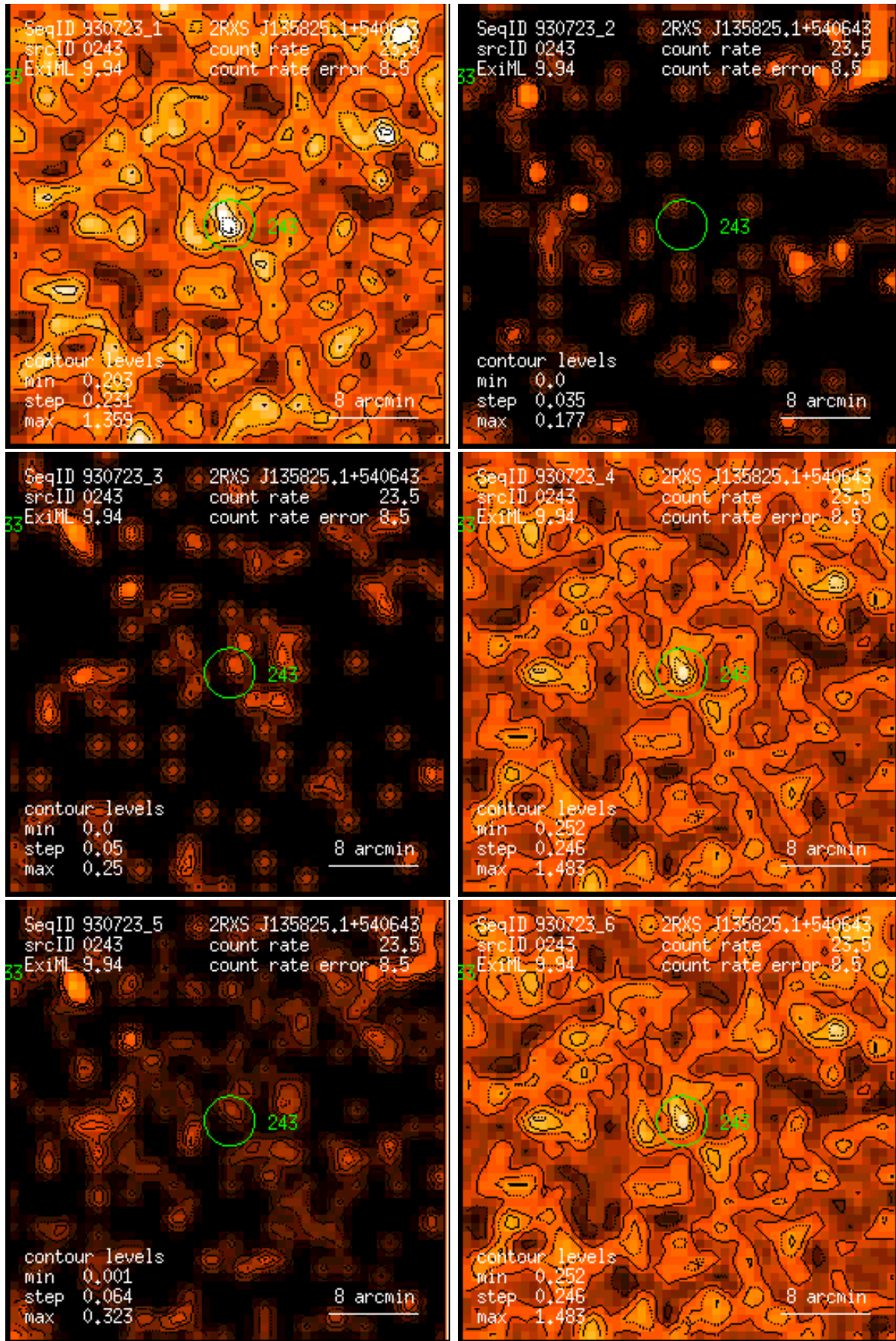
Figure 243: RASS 930723: detection 0243: band rate images, Gaussian filter: (1) PSPC channels 11 – 41, (2) 52 – 90, (3) 91 – 201, (4) 11 – 235, (5) 52 – 201, (6) 11 – 201. Broad band rates in counts/ks. Band rate contour levels in counts/ks/arcmin 2 .
