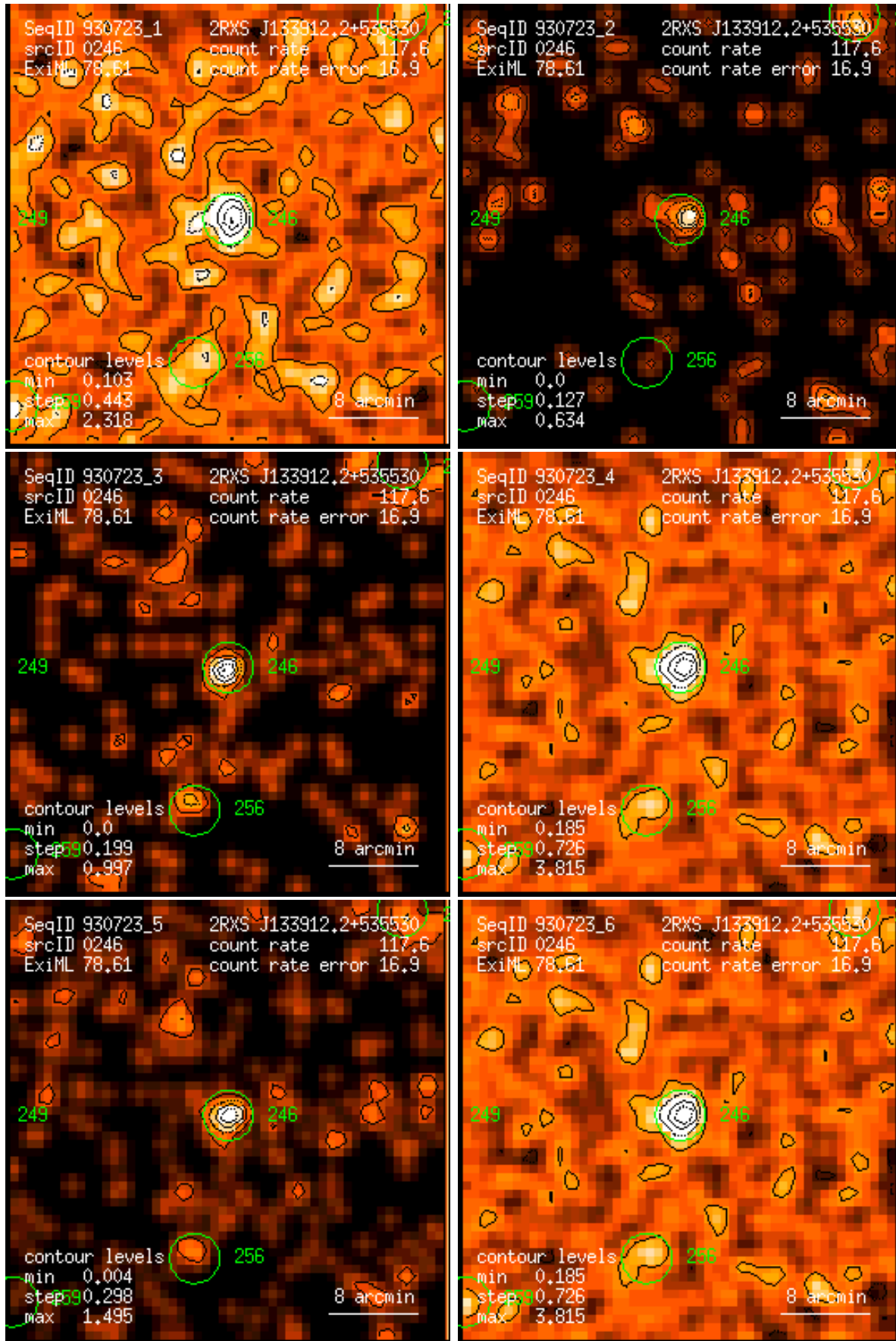
Figure 246: RASS 930723: detection 0246: band rate images, Gaussian filter: (1) PSPC channels 11 – 41, (2) 52 – 90, (3) 91 – 201, (4) 11 – 235, (5) 52 – 201, (6) 11 – 201. Broad band rates in counts/ks. Band rate contour levels in counts/ks/arcmin 2 .
