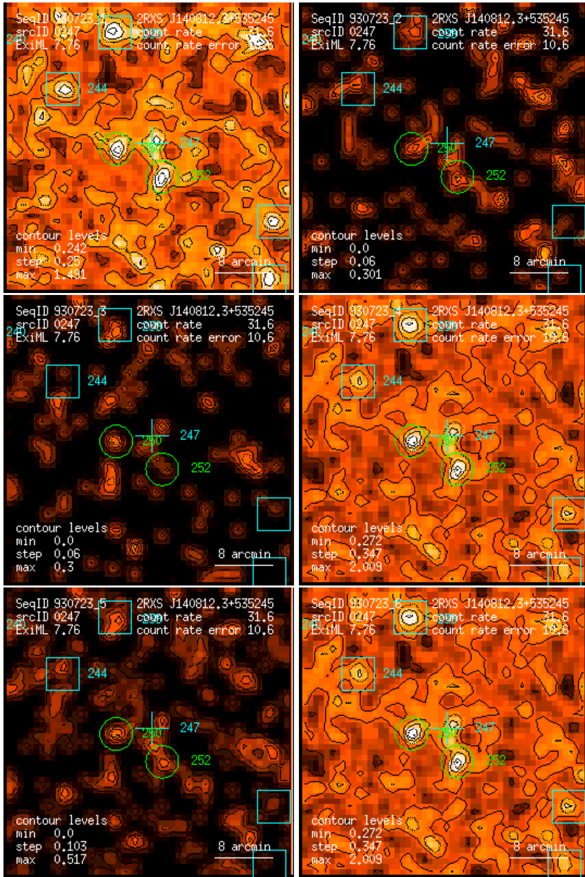
Figure 247: RASS 930723: detection 0247: band rate images, Gaussian filter: (1) PSPC channels 11 – 41, (2) 52 – 90, (3) 91 – 201, (4) 11 – 235, (5) 52 – 201, (6) 11 – 201. Broad band rates in counts/ks. Band rate contour levels in counts/ks/arcmin 2 .
