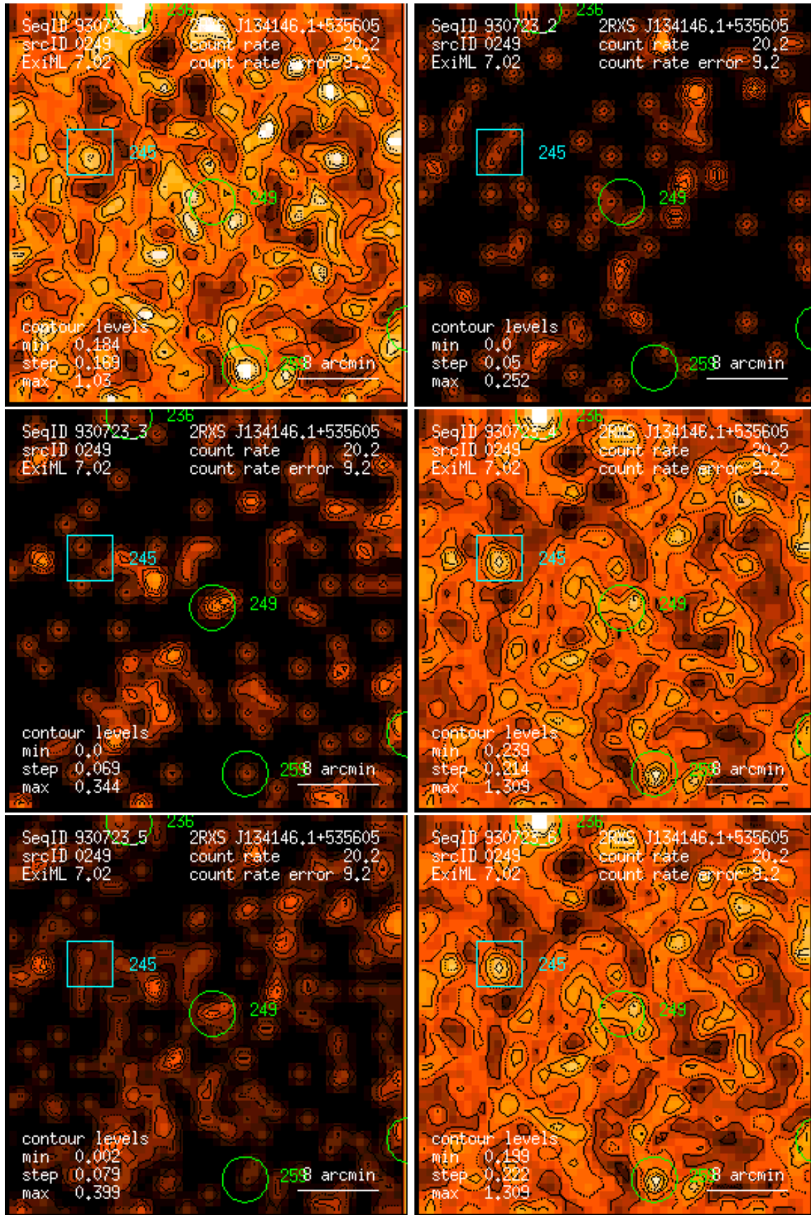
Figure 249: RASS 930723: detection 0249: band rate images, Gaussian filter: (1) PSPC channels 11 – 41, (2) 52 – 90, (3) 91 – 201, (4) 11 – 235, (5) 52 – 201, (6) 11 – 201. Broad band rates in counts/ks. Band rate contour levels in counts/ks/arcmin 2 .
