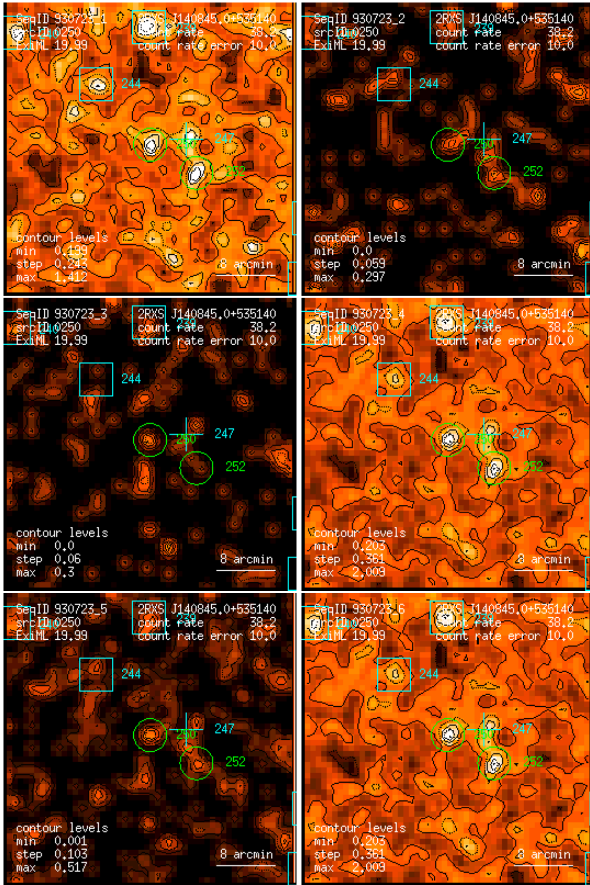
Figure 250: RASS 930723: detection 0250: band rate images, Gaussian filter: (1) PSPC channels 11 – 41, (2) 52 – 90, (3) 91 – 201, (4) 11 – 235, (5) 52 – 201, (6) 11 – 201. Broad band rates in counts/ks. Band rate contour levels in counts/ks/arcmin 2 .
