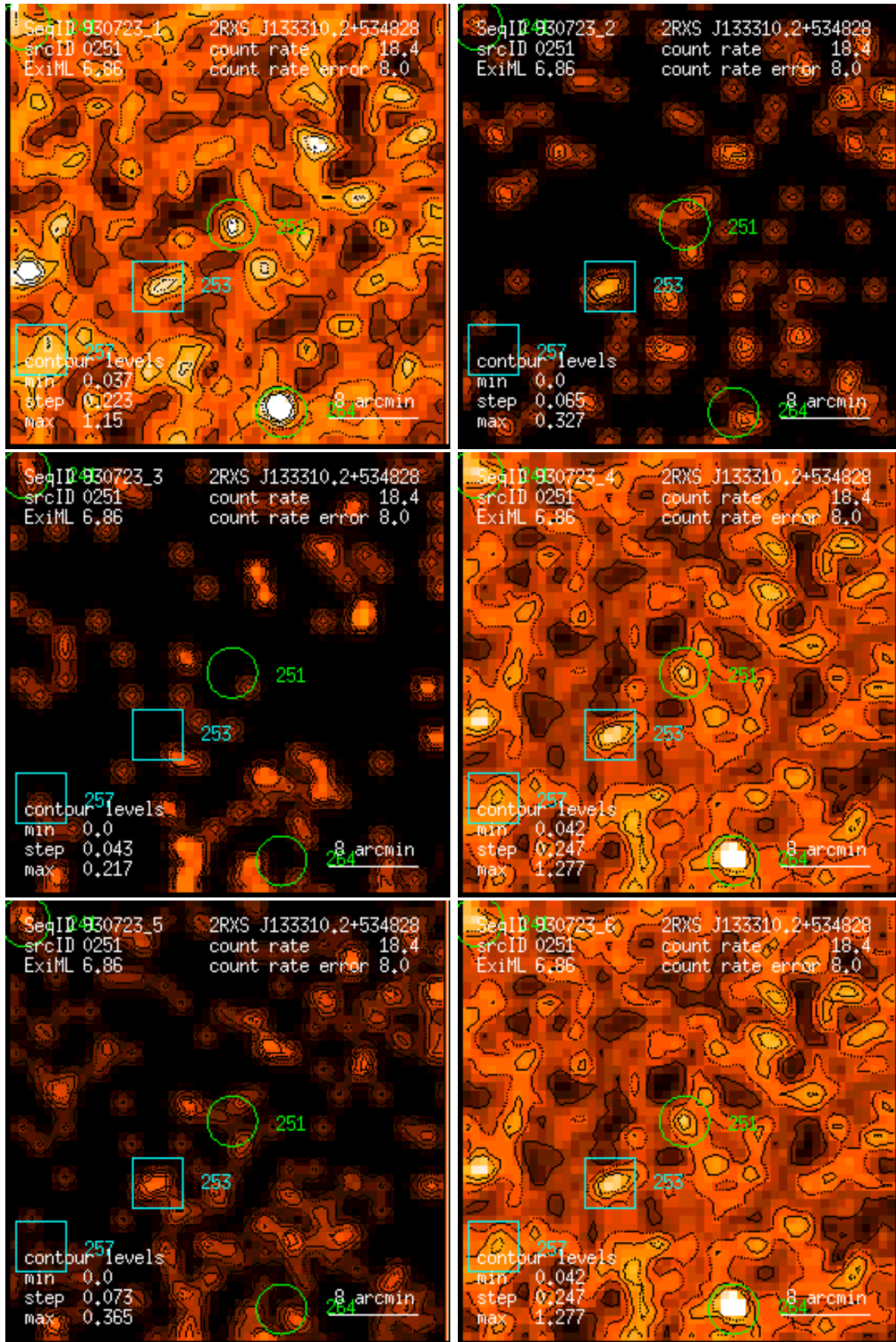
Figure 251: RASS 930723: detection 0251: band rate images, Gaussian filter: (1) PSPC channels 11 – 41, (2) 52 – 90, (3) 91 – 201, (4) 11 – 235, (5) 52 – 201, (6) 11 – 201. Broad band rates in counts/ks. Band rate contour levels in counts/ks/arcmin 2 .
