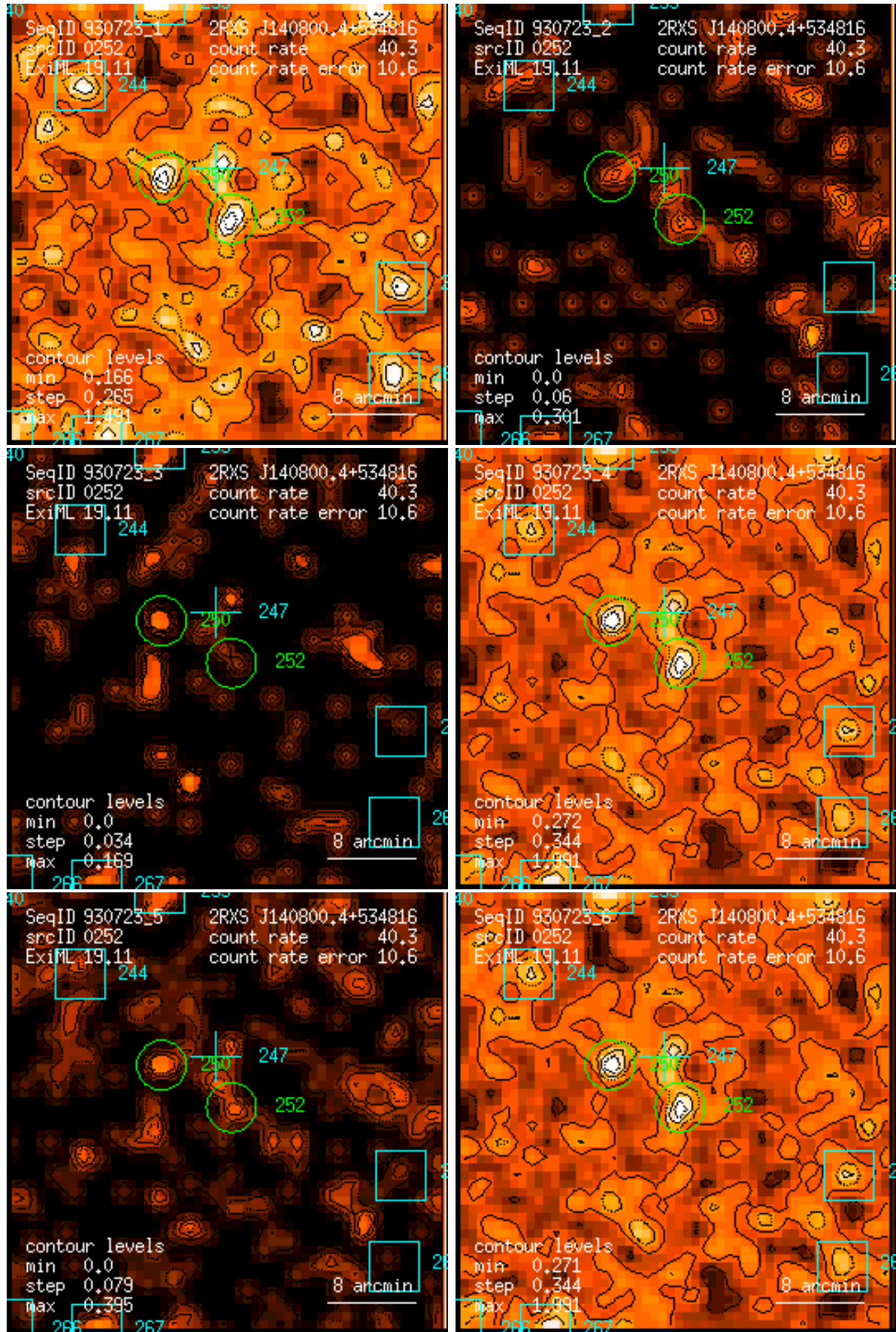
Figure 252: RASS 930723: detection 0252: band rate images, Gaussian filter: (1) PSPC channels 11 – 41, (2) 52 – 90, (3) 91 – 201, (4) 11 – 235, (5) 52 – 201, (6) 11 – 201. Broad band rates in counts/ks. Band rate contour levels in counts/ks/arcmin 2 .
