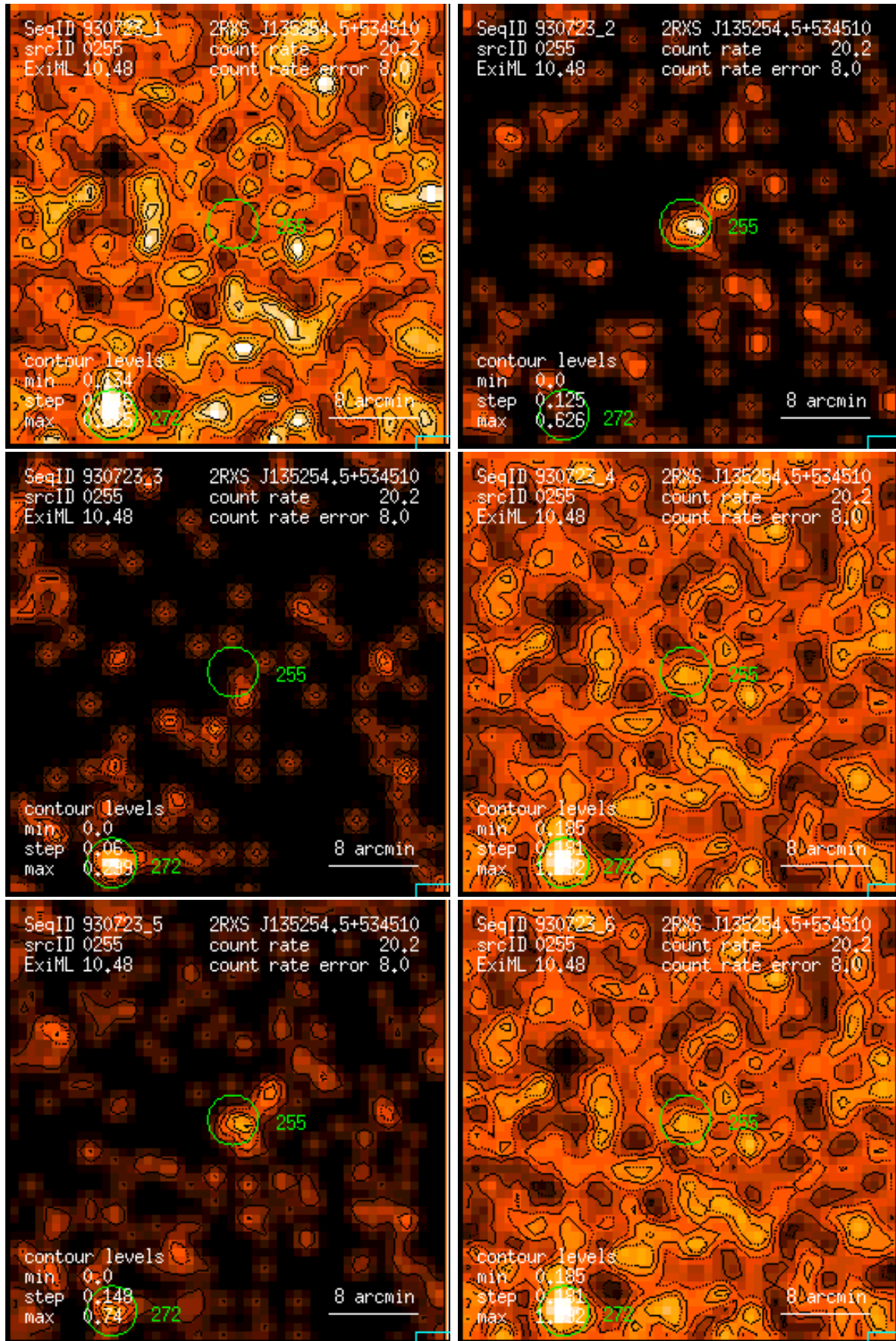
Figure 255: RASS 930723: detection 0255: band rate images, Gaussian filter: (1) PSPC channels 11 – 41, (2) 52 – 90, (3) 91 – 201, (4) 11 – 235, (5) 52 – 201, (6) 11 – 201. Broad band rates in counts/ks. Band rate contour levels in counts/ks/arcmin 2 .
