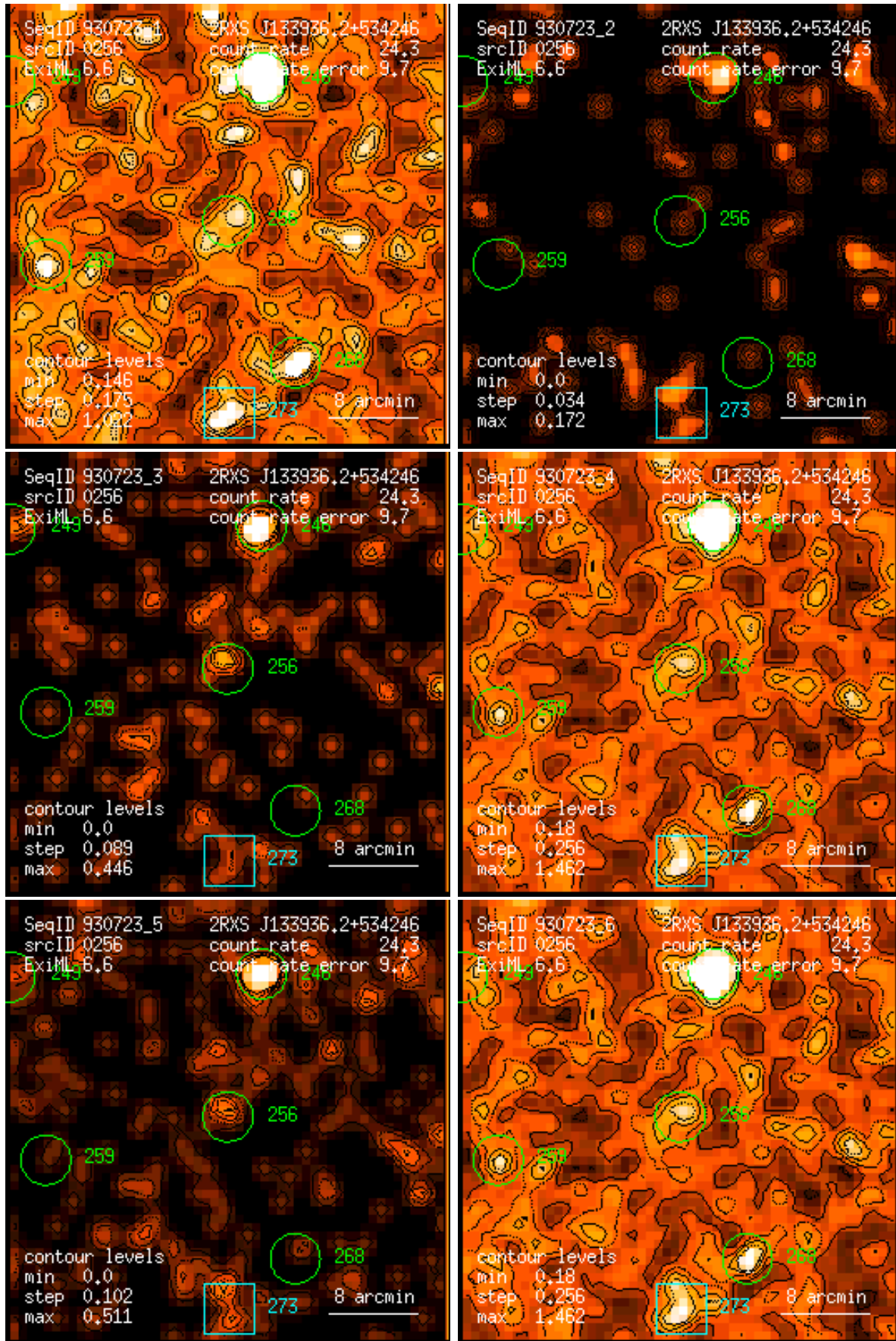
Figure 256: RASS 930723: detection 0256: band rate images, Gaussian filter: (1) PSPC channels 11 – 41, (2) 52 – 90, (3) 91 – 201, (4) 11 – 235, (5) 52 – 201, (6) 11 – 201. Broad band rates in counts/ks. Band rate contour levels in counts/ks/arcmin 2 .
