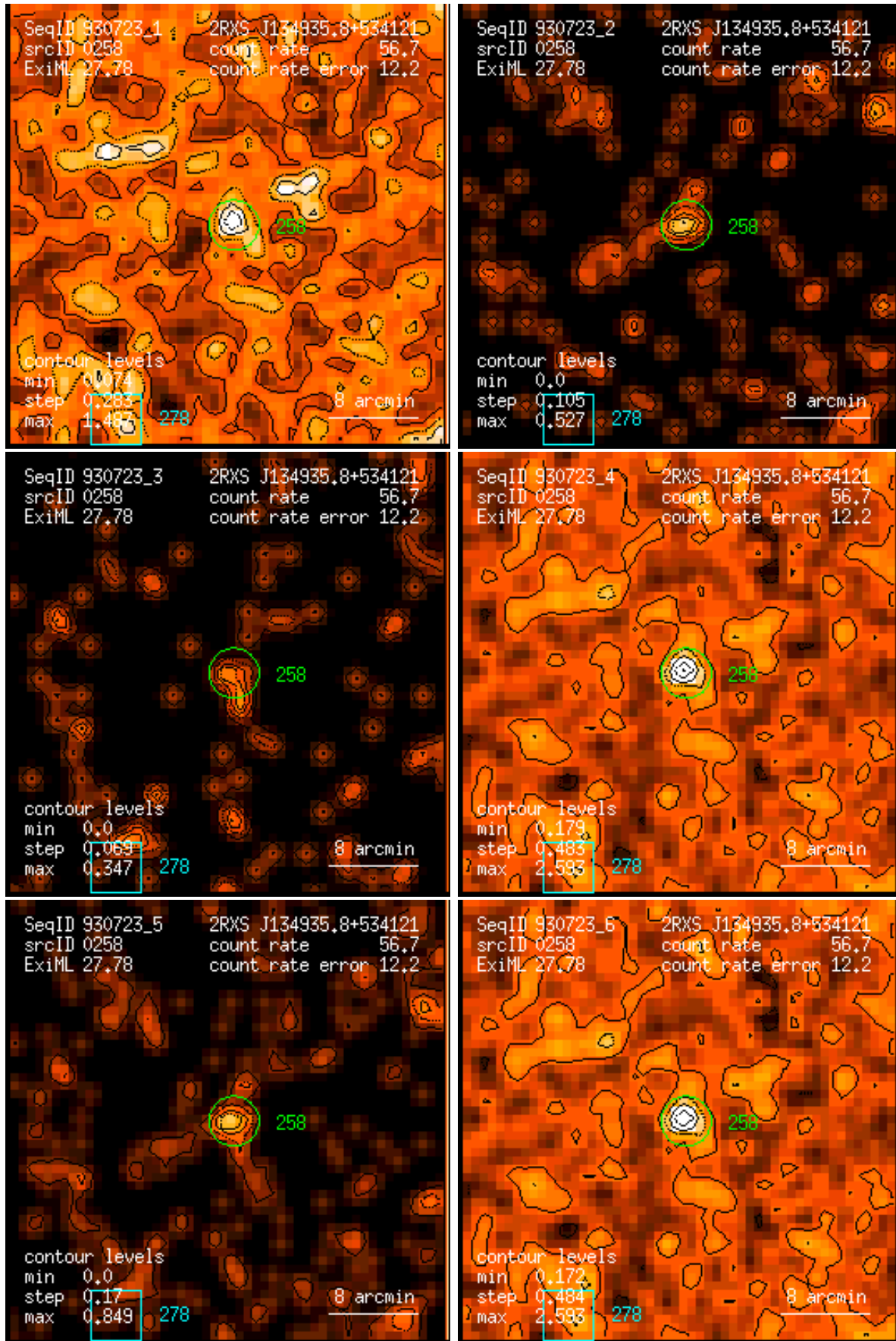
Figure 258: RASS 930723: detection 0258: band rate images, Gaussian filter: (1) PSPC channels 11 – 41, (2) 52 – 90, (3) 91 – 201, (4) 11 – 235, (5) 52 – 201, (6) 11 – 201. Broad band rates in counts/ks. Band rate contour levels in counts/ks/arcmin 2 .
