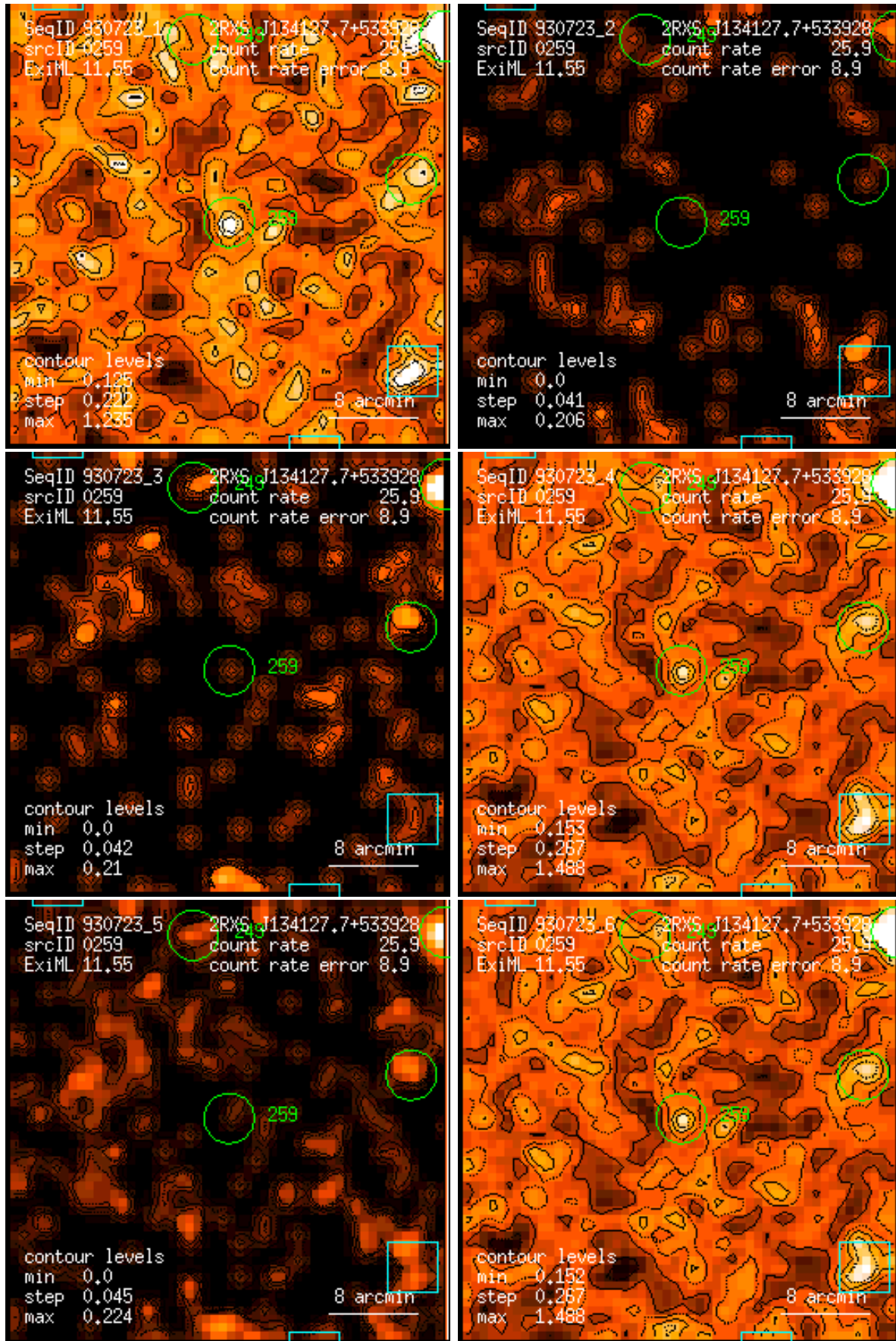
Figure 259: RASS 930723: detection 0259: band rate images, Gaussian filter: (1) PSPC channels 11 – 41, (2) 52 – 90, (3) 91 – 201, (4) 11 – 235, (5) 52 – 201, (6) 11 – 201. Broad band rates in counts/ks. Band rate contour levels in counts/ks/arcmin 2 .
