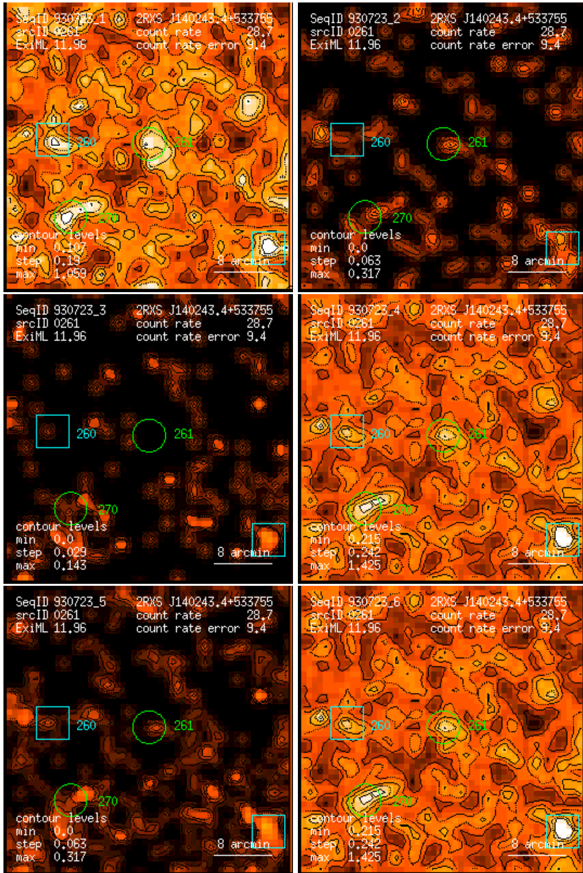
Figure 261: RASS 930723: detection 0261: band rate images, Gaussian filter: (1) PSPC channels 11 – 41, (2) 52 – 90, (3) 91 – 201, (4) 11 – 235, (5) 52 – 201, (6) 11 – 201. Broad band rates in counts/ks. Band rate contour levels in counts/ks/arcmin 2 .
