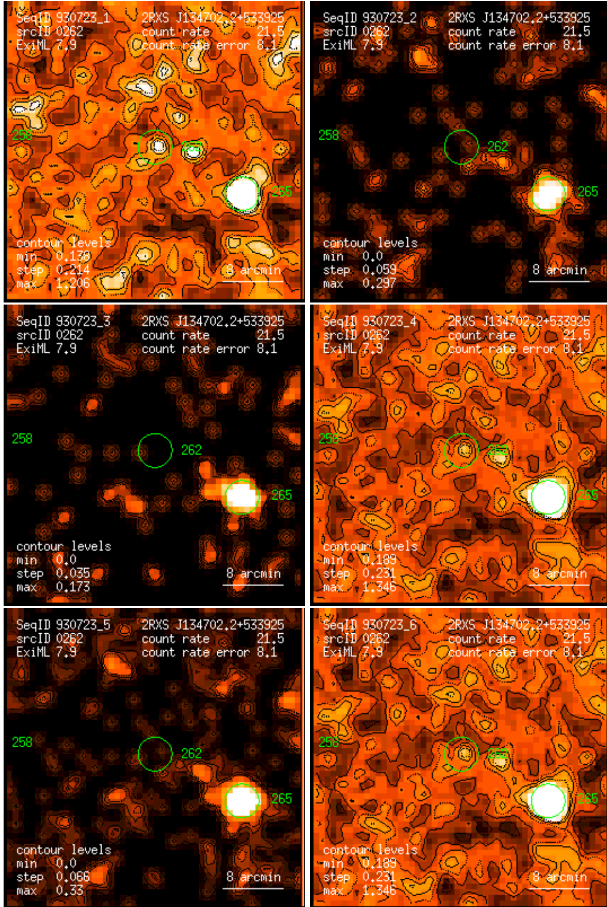
Figure 262: RASS 930723: detection 0262: band rate images, Gaussian filter: (1) PSPC channels 11 – 41, (2) 52 – 90, (3) 91 – 201, (4) 11 – 235, (5) 52 – 201, (6) 11 – 201. Broad band rates in counts/ks. Band rate contour levels in counts/ks/arcmin 2 .
