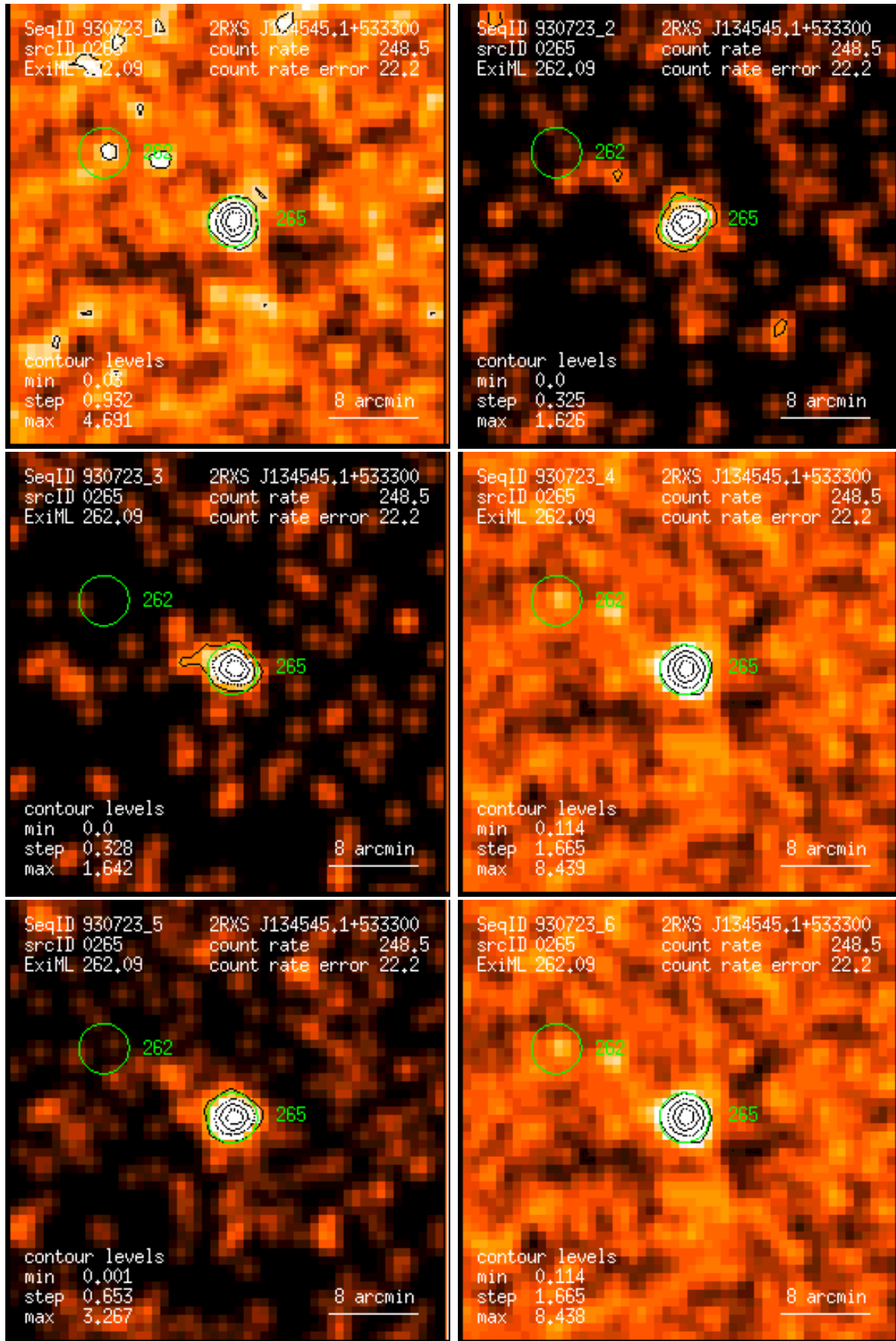
Figure 265: RASS 930723: detection 0265: band rate images, Gaussian filter: (1) PSPC channels 11 – 41, (2) 52 – 90, (3) 91 – 201, (4) 11 – 235, (5) 52 – 201, (6) 11 – 201. Broad band rates in counts/ks. Band rate contour levels in counts/ks/arcmin 2 .
