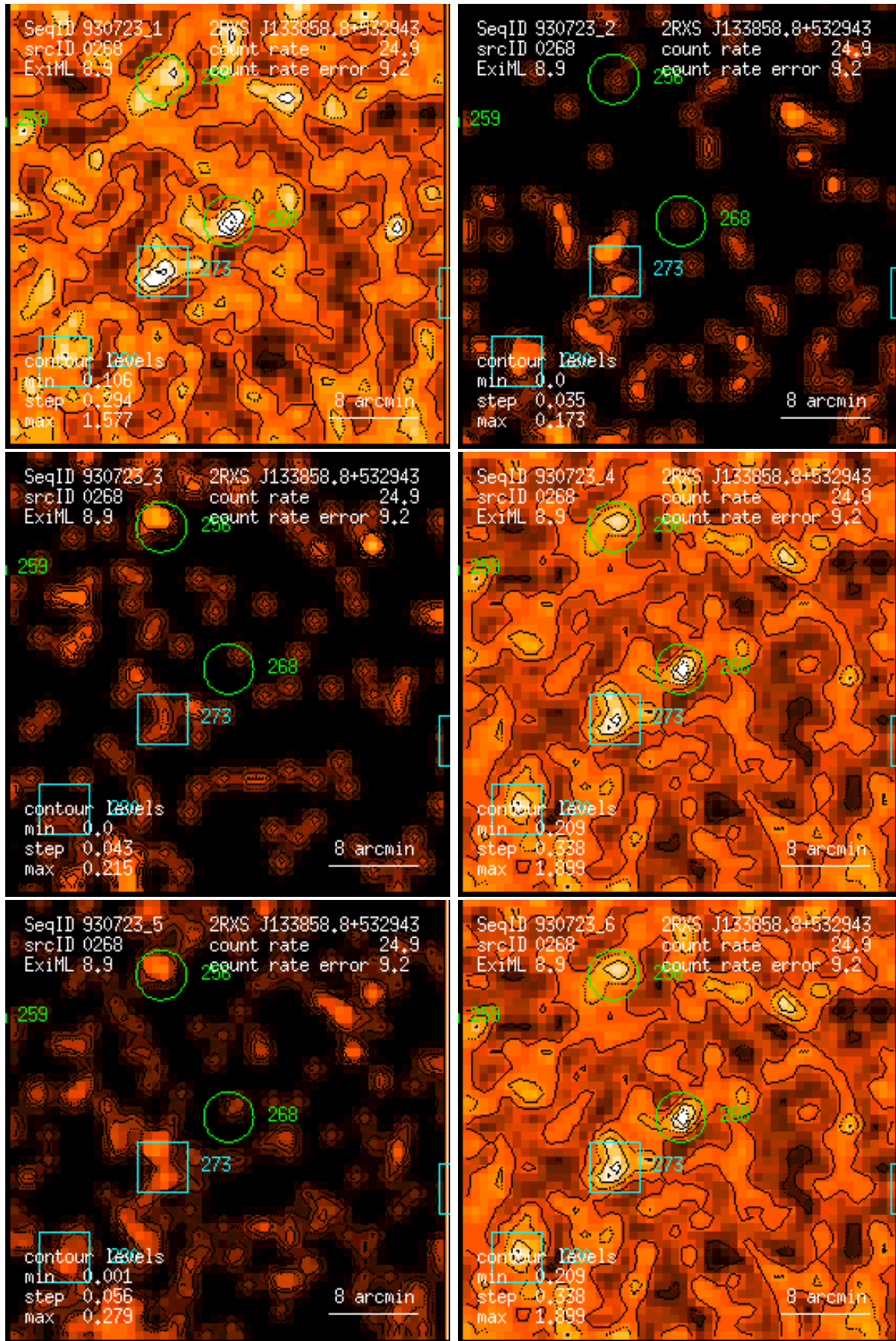
Figure 268: RASS 930723: detection 0268: band rate images, Gaussian filter: (1) PSPC channels 11 – 41, (2) 52 – 90, (3) 91 – 201, (4) 11 – 235, (5) 52 – 201, (6) 11 – 201. Broad band rates in counts/ks. Band rate contour levels in counts/ks/arcmin 2 .
