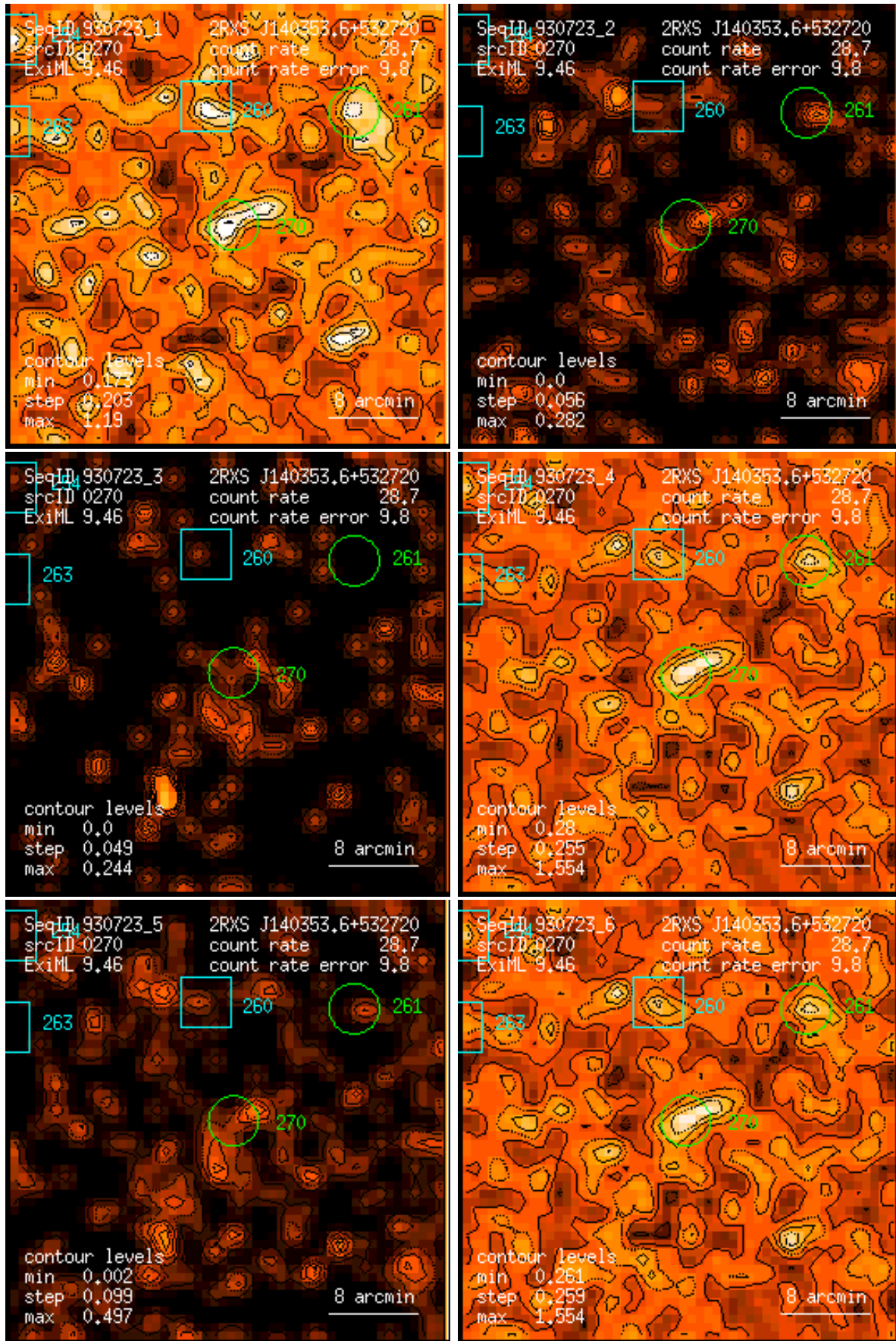
Figure 270: RASS 930723: detection 0270: band rate images, Gaussian filter: (1) PSPC channels 11 – 41, (2) 52 – 90, (3) 91 – 201, (4) 11 – 235, (5) 52 – 201, (6) 11 – 201. Broad band rates in counts/ks. Band rate contour levels in counts/ks/arcmin 2 .
