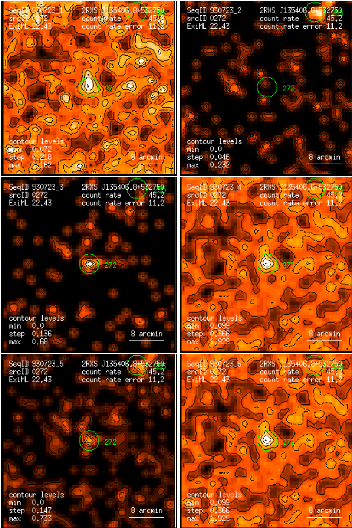
Figure 272: RASS 930723: detection 0272: band rate images, Gaussian filter: (1) PSPC channels 11 – 41, (2) 52 – 90, (3) 91 – 201, (4) 11 – 235, (5) 52 – 201, (6) 11 – 201. Broad band rates in counts/ks. Band rate contour levels in counts/ks/arcmin 2 .
