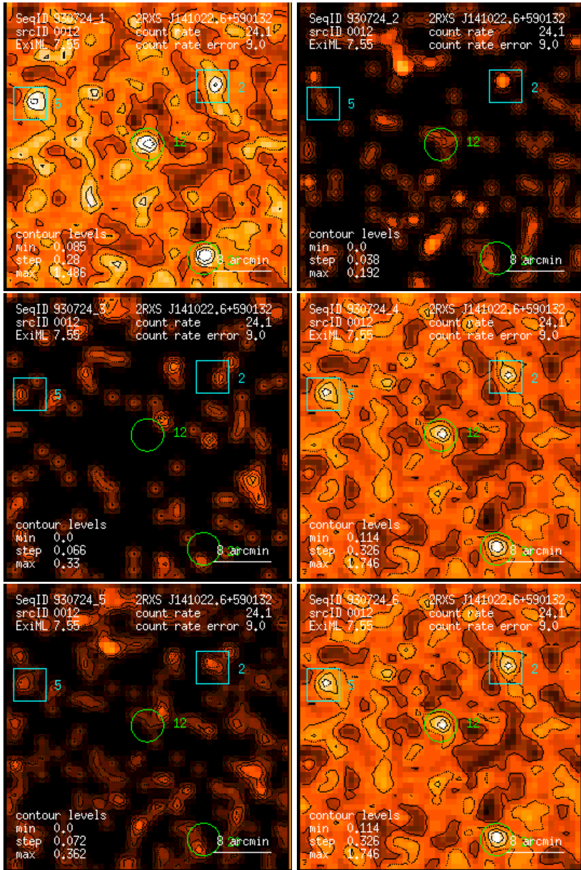
Figure 12: RASS 930724: detection 0012: band rate images, Gaussian filter: (1) PSPC channels 11 – 41, (2) 52 – 90, (3) 91 – 201, (4) 11 – 235, (5) 52 – 201, (6) 11 – 201. Broad band rates in counts/ks. Band rate contour levels in counts/ks/arcmin 2 .
