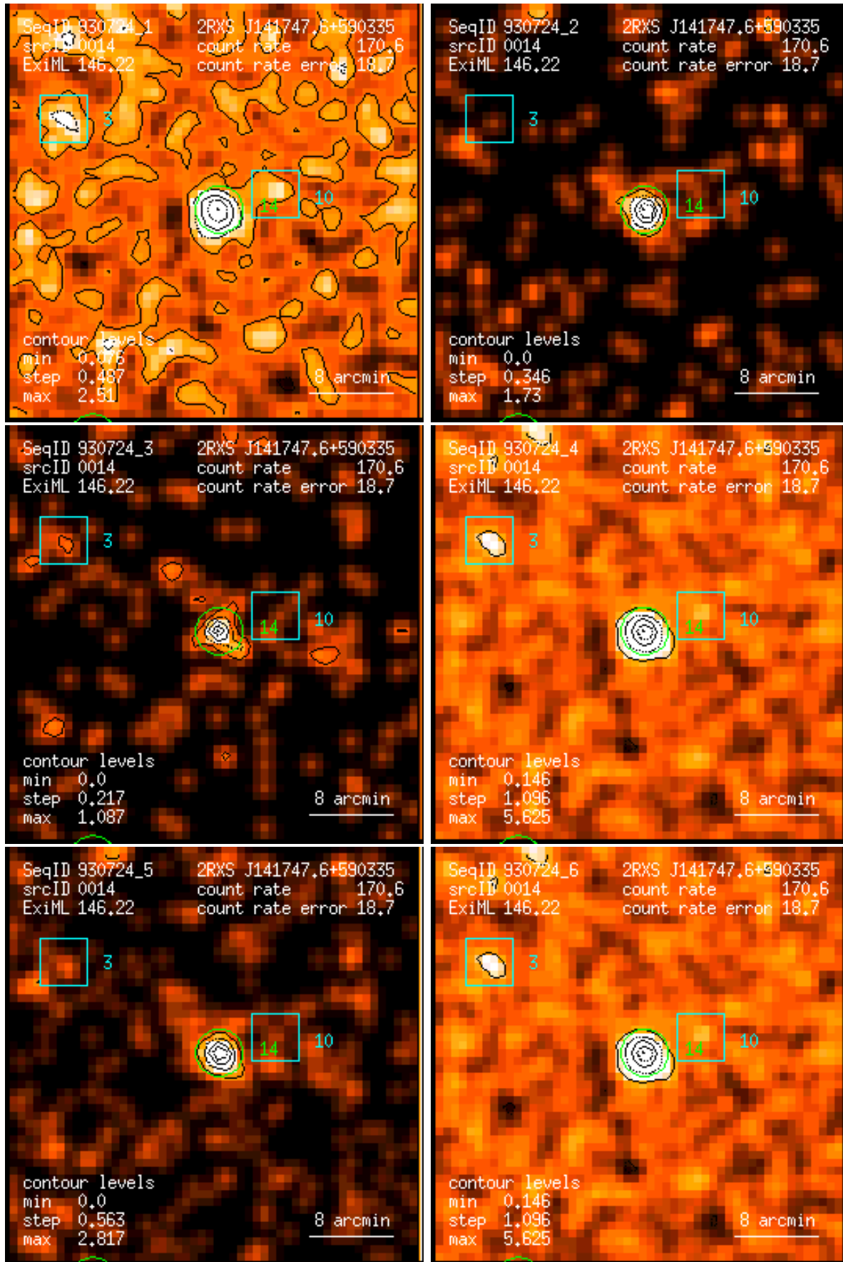
Figure 14: RASS 930724: detection 0014: band rate images, Gaussian filter: (1) PSPC channels 11 – 41, (2) 52 – 90, (3) 91 – 201, (4) 11 – 235, (5) 52 – 201, (6) 11 – 201. Broad band rates in counts/ks. Band rate contour levels in counts/ks/arcmin 2 .
