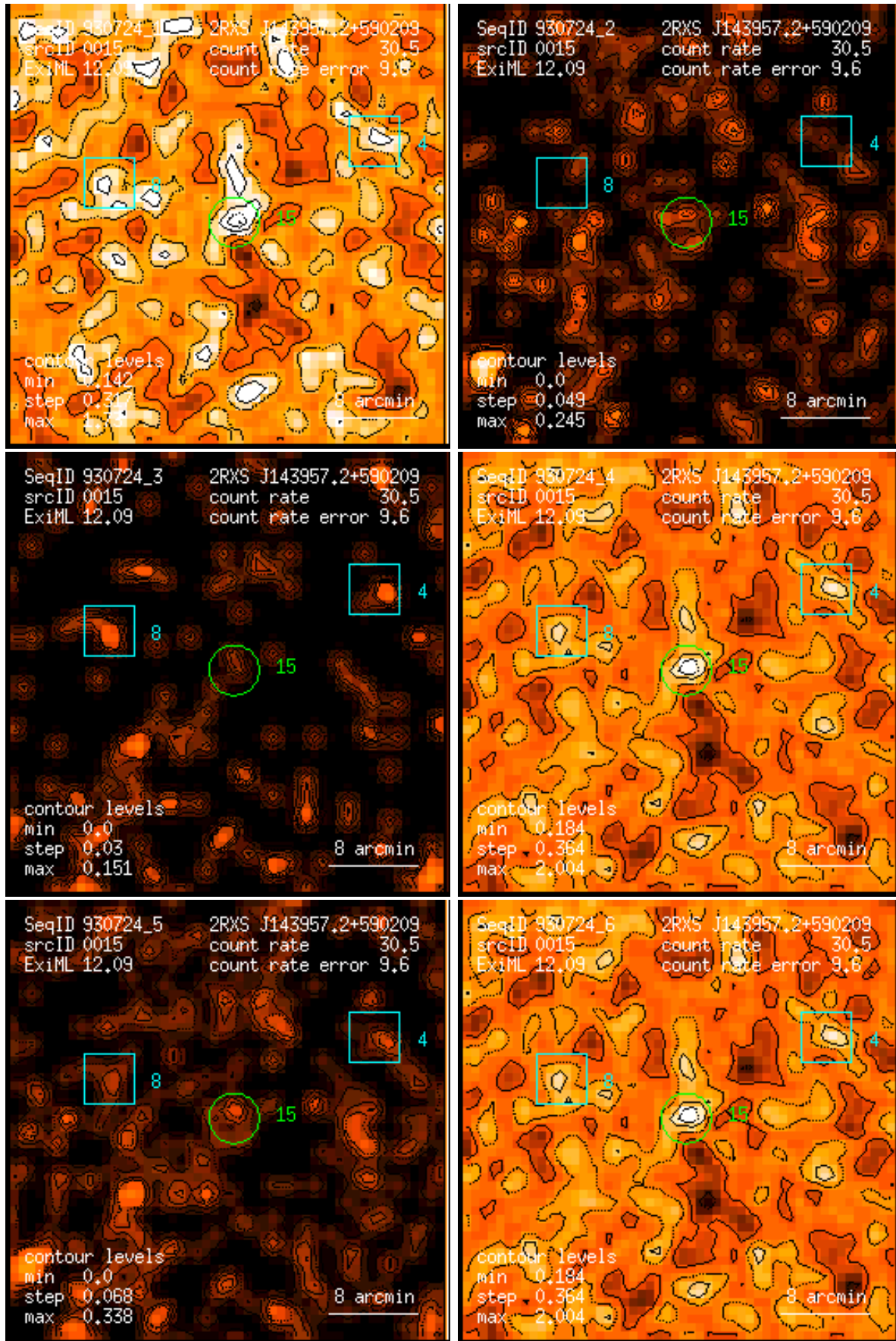
Figure 15: RASS 930724: detection 0015: band rate images, Gaussian filter: (1) PSPC channels 11 – 41, (2) 52 – 90, (3) 91 – 201, (4) 11 – 235, (5) 52 – 201, (6) 11 – 201. Broad band rates in counts/ks. Band rate contour levels in counts/ks/arcmin 2 .
