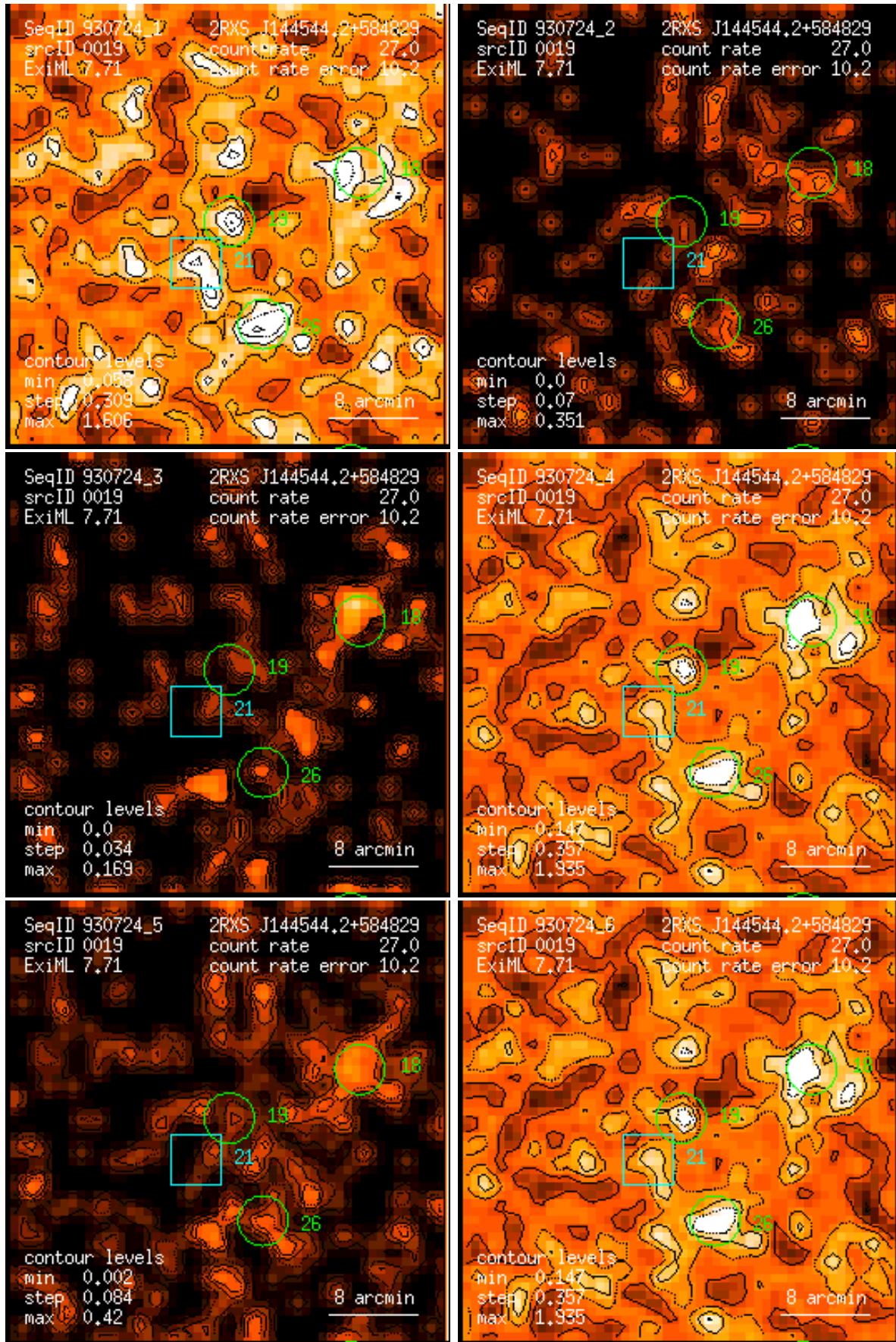
Figure 19: RASS 930724: detection 0019: band rate images, Gaussian filter: (1) PSPC channels 11 – 41, (2) 52 – 90, (3) 91 – 201, (4) 11 – 235, (5) 52 – 201, (6) 11 – 201. Broad band rates in counts/ks. Band rate contour levels in counts/ks/arcmin 2 .
