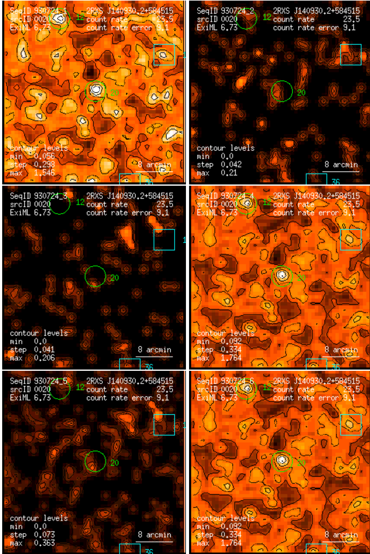
Figure 20: RASS 930724: detection 0020: band rate images, Gaussian filter: (1) PSPC channels 11 – 41, (2) 52 – 90, (3) 91 – 201, (4) 11 – 235, (5) 52 – 201, (6) 11 – 201. Broad band rates in counts/ks. Band rate contour levels in counts/ks/arcmin 2 .
