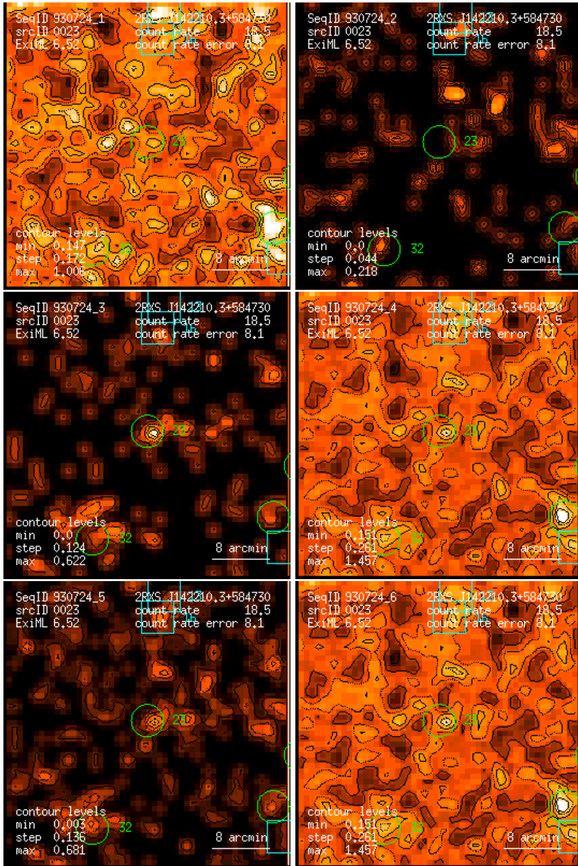
Figure 23: RASS 930724: detection 0023: band rate images, Gaussian filter: (1) PSPC channels 11 – 41, (2) 52 – 90, (3) 91 – 201, (4) 11 – 235, (5) 52 – 201, (6) 11 – 201. Broad band rates in counts/ks. Band rate contour levels in counts/ks/arcmin 2 .
