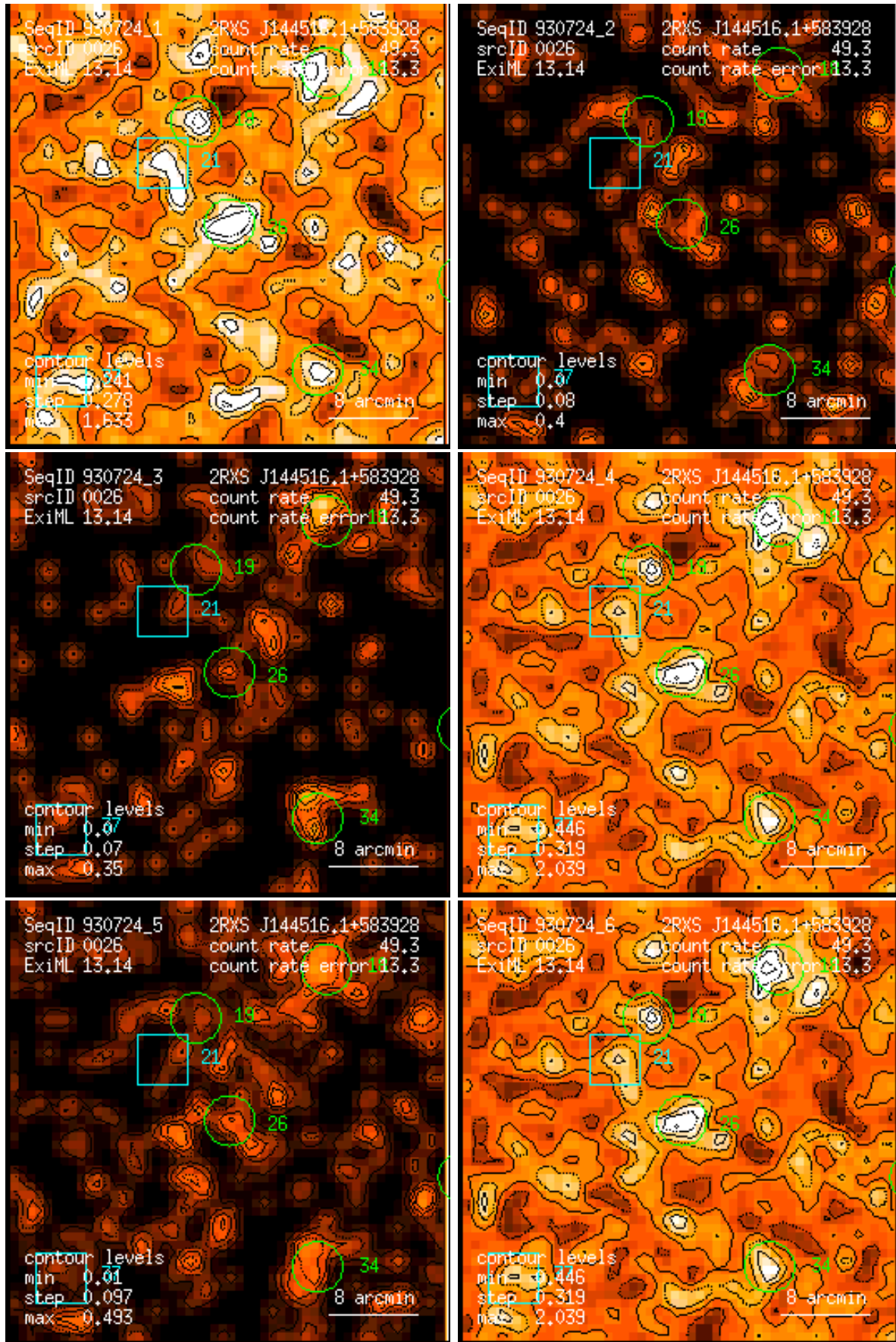
Figure 26: RASS 930724: detection 0026: band rate images, Gaussian filter: (1) PSPC channels 11 – 41, (2) 52 – 90, (3) 91 – 201, (4) 11 – 235, (5) 52 – 201, (6) 11 – 201. Broad band rates in counts/ks. Band rate contour levels in counts/ks/arcmin 2 .
