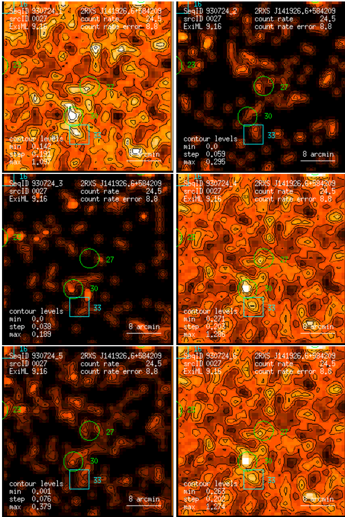
Figure 27: RASS 930724: detection 0027: band rate images, Gaussian filter: (1) PSPC channels 11 – 41, (2) 52 – 90, (3) 91 – 201, (4) 11 – 235, (5) 52 – 201, (6) 11 – 201. Broad band rates in counts/ks. Band rate contour levels in counts/ks/arcmin 2 .
