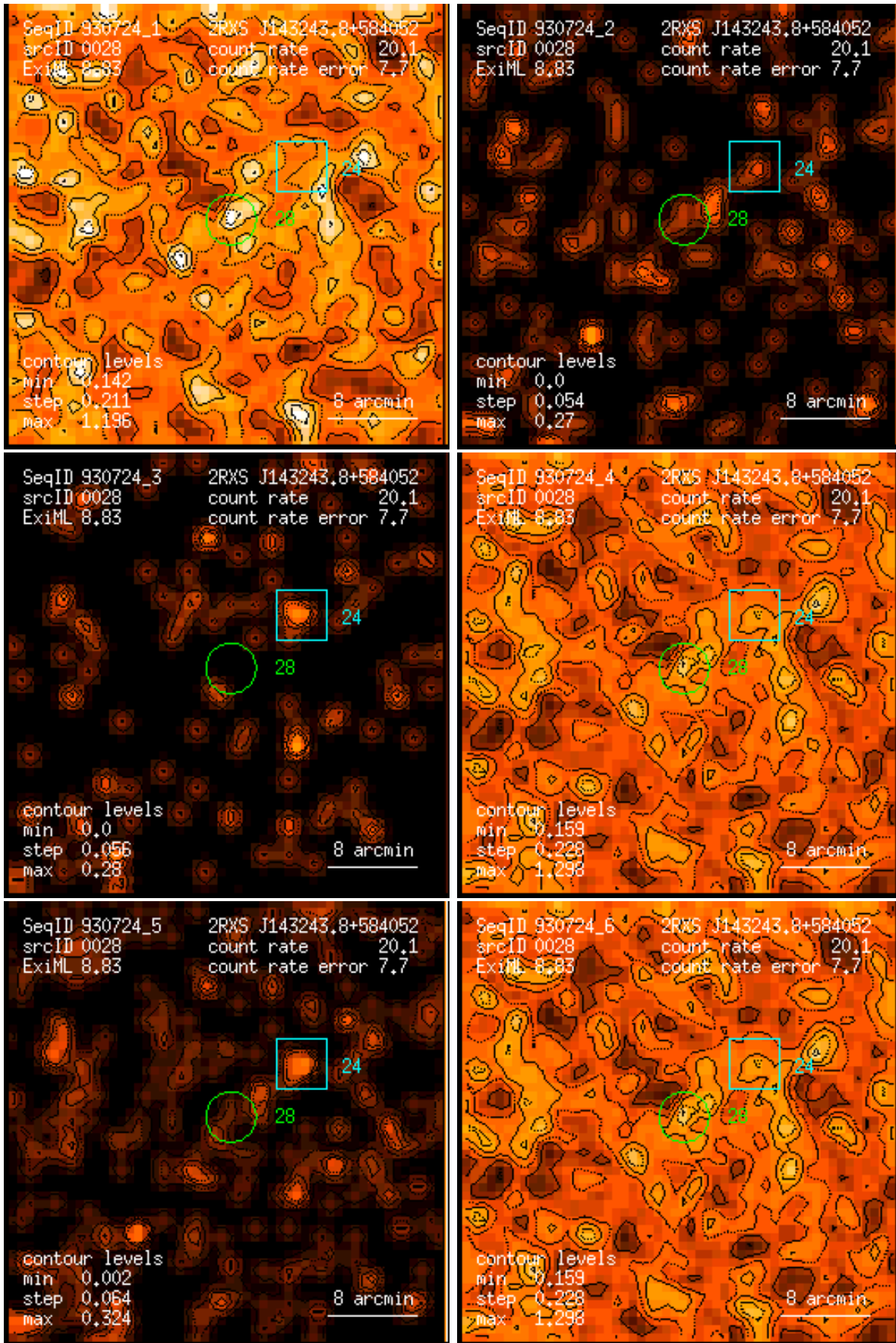
Figure 28: RASS 930724: detection 0028: band rate images, Gaussian filter: (1) PSPC channels 11 – 41, (2) 52 – 90, (3) 91 – 201, (4) 11 – 235, (5) 52 – 201, (6) 11 – 201. Broad band rates in counts/ks. Band rate contour levels in counts/ks/arcmin 2 .
