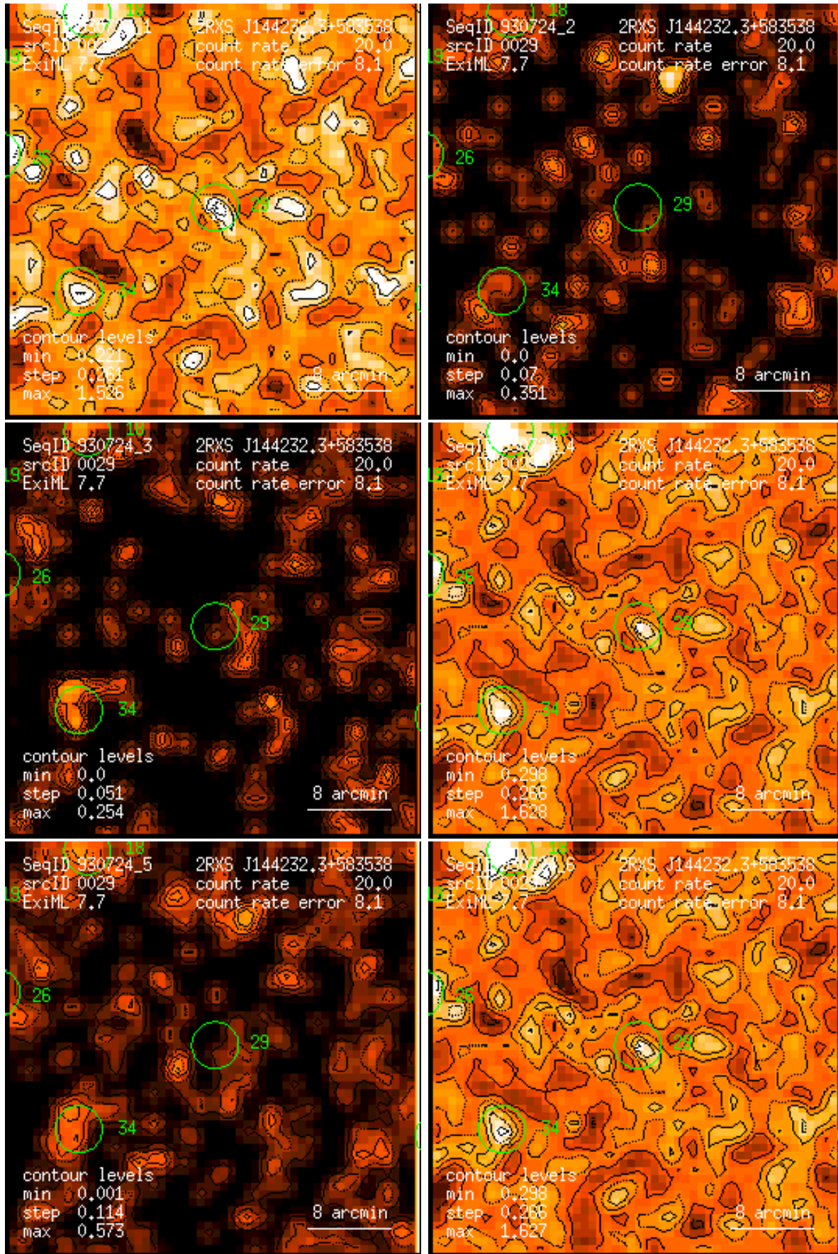
Figure 29: RASS 930724: detection 0029: band rate images, Gaussian filter: (1) PSPC channels 11 – 41, (2) 52 – 90, (3) 91 – 201, (4) 11 – 235, (5) 52 – 201, (6) 11 – 201. Broad band rates in counts/ks. Band rate contour levels in counts/ks/arcmin 2 .
