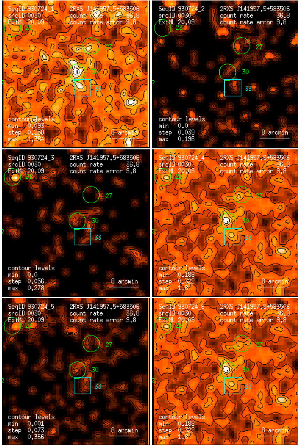
Figure 30: RASS 930724: detection 0030: band rate images, Gaussian filter: (1) PSPC channels 11 – 41, (2) 52 – 90, (3) 91 – 201, (4) 11 – 235, (5) 52 – 201, (6) 11 – 201. Broad band rates in counts/ks. Band rate contour levels in counts/ks/arcmin 2 .
