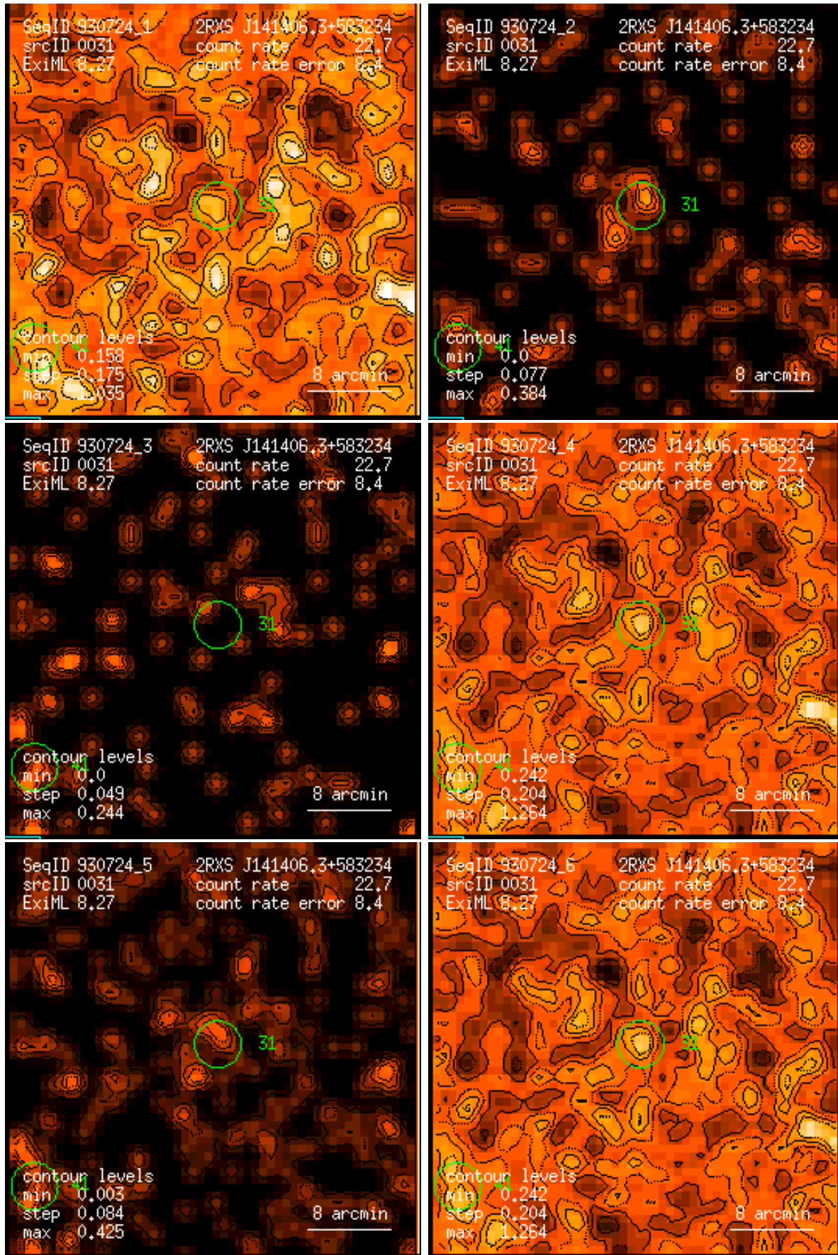
Figure 31: RASS 930724: detection 0031: band rate images, Gaussian filter: (1) PSPC channels 11 – 41, (2) 52 – 90, (3) 91 – 201, (4) 11 – 235, (5) 52 – 201, (6) 11 – 201. Broad band rates in counts/ks. Band rate contour levels in counts/ks/arcmin 2 .
