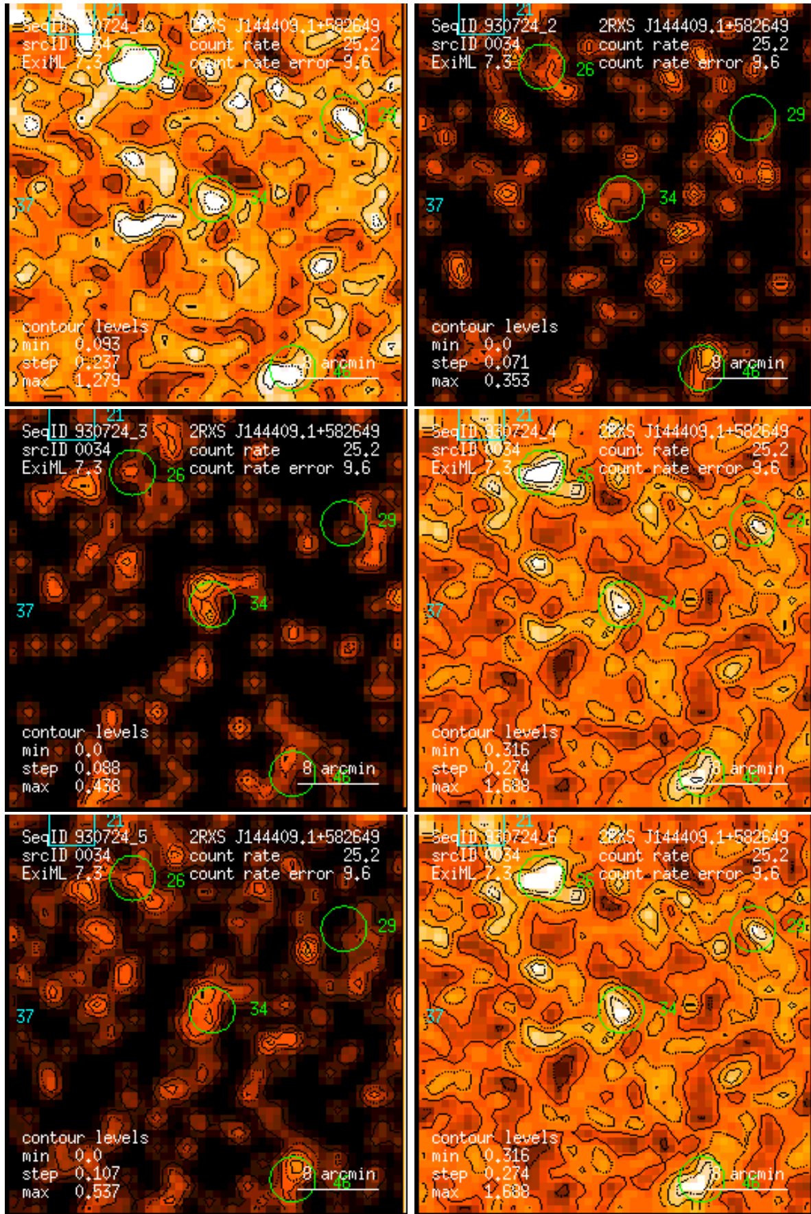
Figure 34: RASS 930724: detection 0034: band rate images, Gaussian filter: (1) PSPC channels 11 – 41, (2) 52 – 90, (3) 91 – 201, (4) 11 – 235, (5) 52 – 201, (6) 11 – 201. Broad band rates in counts/ks. Band rate contour levels in counts/ks/arcmin 2 .
