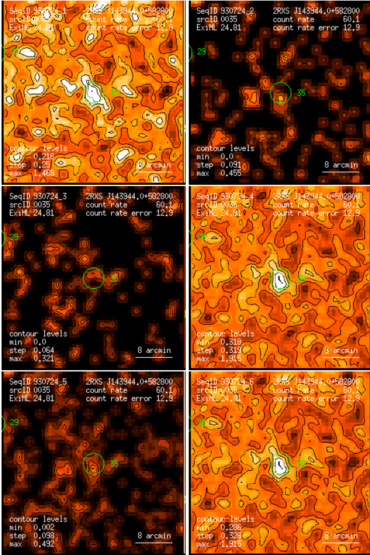
Figure 35: RASS 930724: detection 0035: band rate images, Gaussian filter: (1) PSPC channels 11 – 41, (2) 52 – 90, (3) 91 – 201, (4) 11 – 235, (5) 52 – 201, (6) 11 – 201. Broad band rates in counts/ks. Band rate contour levels in counts/ks/arcmin 2 .
