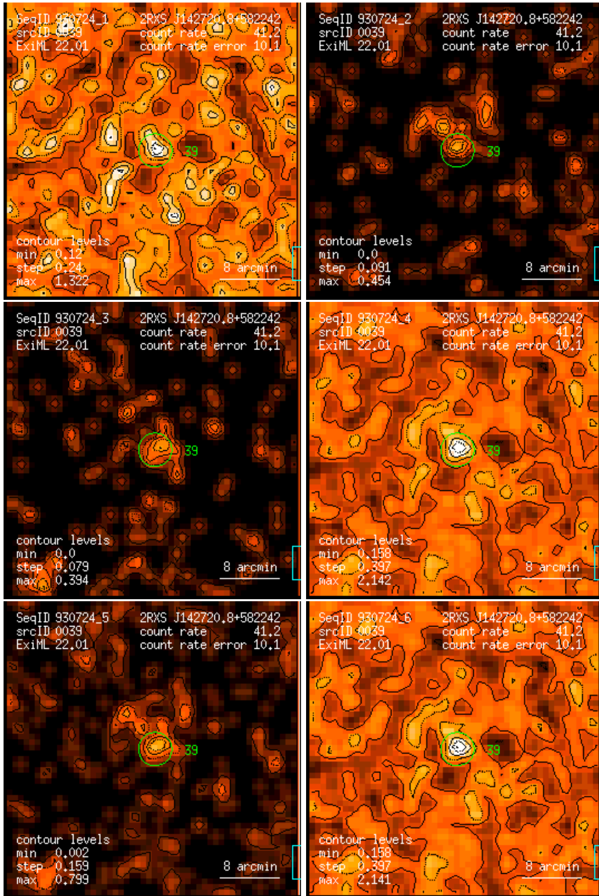
Figure 39: RASS 930724: detection 0039: band rate images, Gaussian filter: (1) PSPC channels 11 – 41, (2) 52 – 90, (3) 91 – 201, (4) 11 – 235, (5) 52 – 201, (6) 11 – 201. Broad band rates in counts/ks. Band rate contour levels in counts/ks/arcmin 2 .
