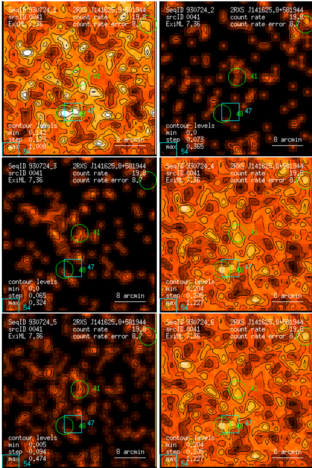
Figure 41: RASS 930724: detection 0041: band rate images, Gaussian filter: (1) PSPC channels 11 – 41, (2) 52 – 90, (3) 91 – 201, (4) 11 – 235, (5) 52 – 201, (6) 11 – 201. Broad band rates in counts/ks. Band rate contour levels in counts/ks/arcmin 2 .
