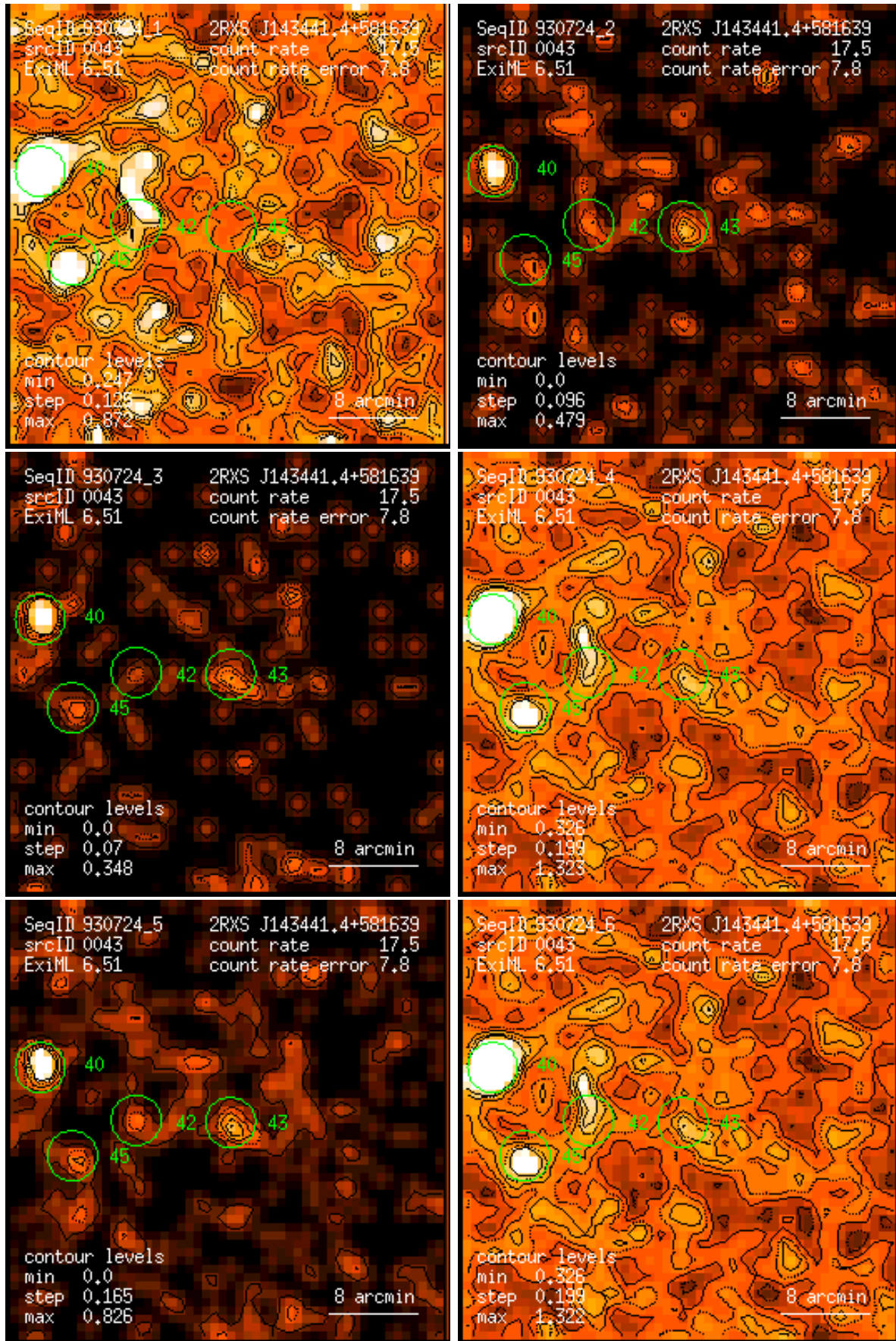
Figure 43: RASS 930724: detection 0043: band rate images, Gaussian filter: (1) PSPC channels 11 – 41, (2) 52 – 90, (3) 91 – 201, (4) 11 – 235, (5) 52 – 201, (6) 11 – 201. Broad band rates in counts/ks. Band rate contour levels in counts/ks/arcmin 2 .
