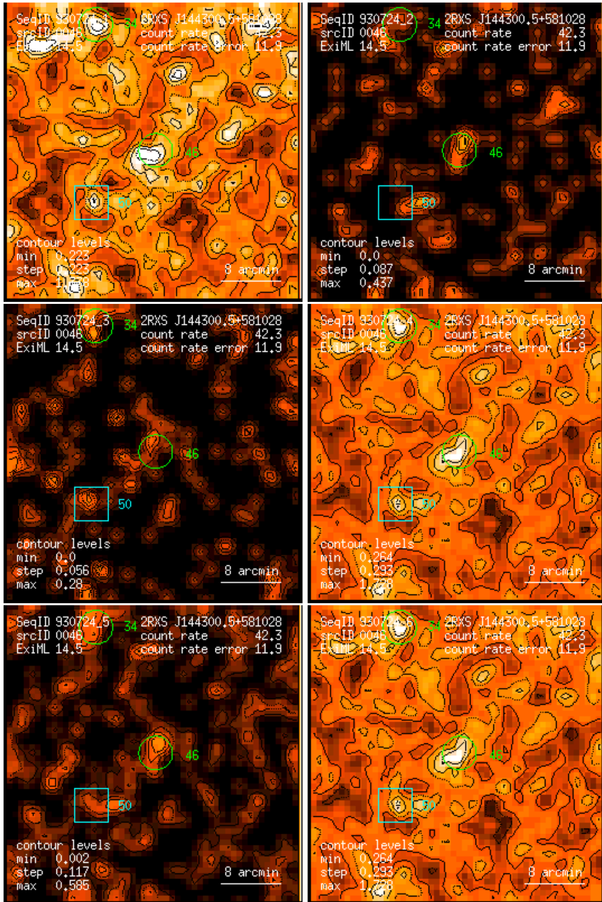
Figure 46: RASS 930724: detection 0046: band rate images, Gaussian filter: (1) PSPC channels 11 – 41, (2) 52 – 90, (3) 91 – 201, (4) 11 – 235, (5) 52 – 201, (6) 11 – 201. Broad band rates in counts/ks. Band rate contour levels in counts/ks/arcmin 2 .
